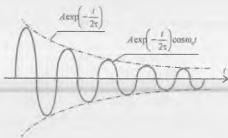
21.1-rasm. Ekspontensial so'nuvchi tebranish jarayon deyarli davriy bo'lib, tebranish chastotasi taxminan \omega_0 ga teng.
