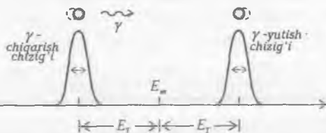
23.5-rasm. Yadroviy nurlanish va yutilish jarayonida yutilish va chiqarish chiziqklarining bir-biriga nisbatan ko'chishi.
