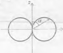
20.5-rasm. Energiyaning burchak taqsimoti.
