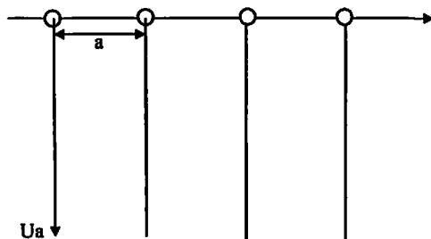
6.7 – rasm. Kristall panjara atomlari potensial energiyalari ko'rinishi
