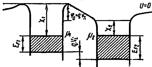
9.4 – rasm. Metall – metall kontaktining energetik diagrammasi
