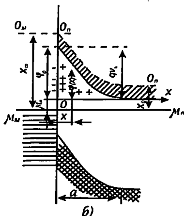
9.8 – rasm. Metall – yarimo'tkazgich kontakti
