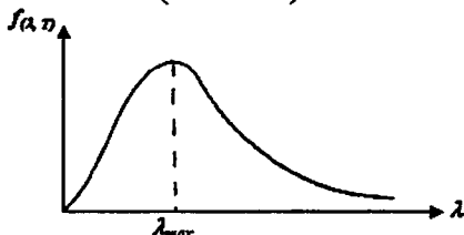
4.2-rasm. Nurlanish spektrining Plank ifodasi
