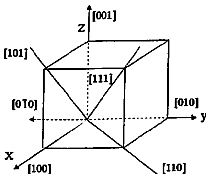
6.6 – rasm. Kristall panjaraning yo'nalishlari
