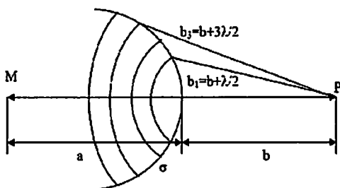
2.2-rasm. Sferik to'liqin frontini Frenel sohalariga ajratish
