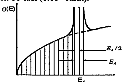
6.16 – rasm. O'tao'tkazuvchanlik holatga o'tishdagi energetik tirqishning hosil bo'lishi
