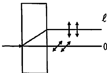
3.6 – rasm. Qo'sh nur sinishi
