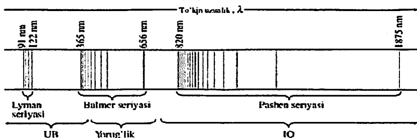
5.1-rasm. Vodorod atomining chiziqli spektri
