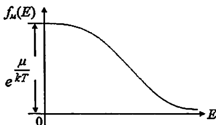
6.1.3 – rasm. Maksvell – Bolsman funksiyasining energiyaga bog'liqligi
