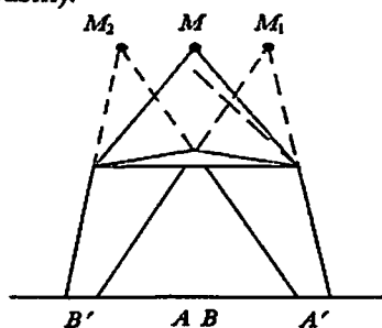
1.5-rasm. Biprizmadagi Frenel tajribasi
