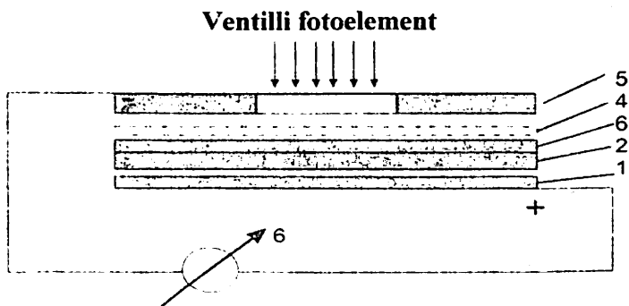
2.2-rasm. Selenli fotoelement
