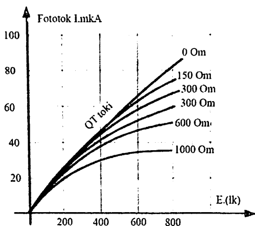
2.3.-rasm. Yorug'lik oqimining o'zgarishi
