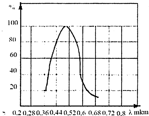
3.3-rasm. Lyuminessensiya spektri
