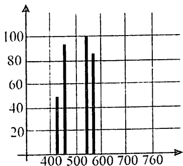
1.2-rasm. Murakkab nurlanish.
