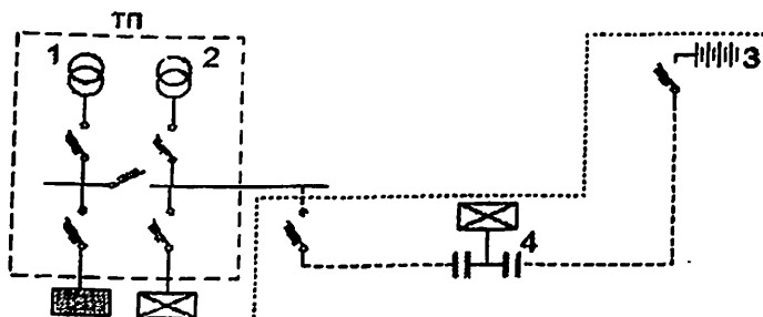
5.7 -rasm. “O‘zgacha” toifali avariya yoritishni ta‘minlash sxemasi.
