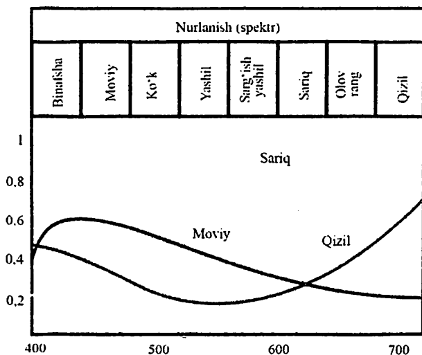
1.14-rasm Nurlanish spektr (ko'k, sariq, qizil)
