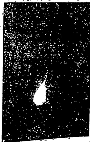
116-rasm. Mashhur Galley kometasi (1986-y.)
