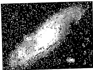
149-rasm. Galaktikamizga qo'shni Andromeda galaktikasi
