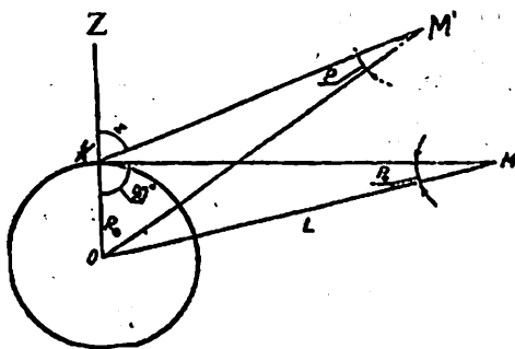
19-rasm. Yoritgichlarning sutkalik va sutkalik-gorizontal parallaksilari
