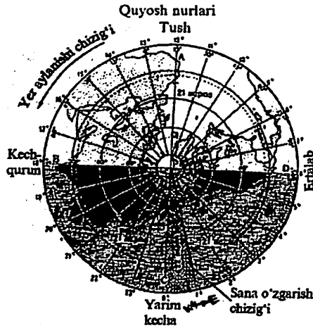
16-rasm. Datani o'zgartirish chizig'i
