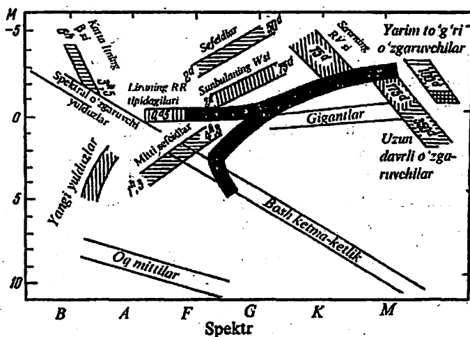
139-rasm. Spektr – yorqinlik diagrammasida sefeidlarning o'zgarishi
