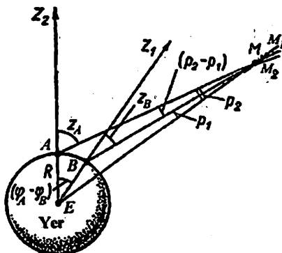
35-rasm. M osmon jismining sutkalik gorizontal parallaksini hisoblash
