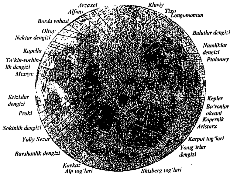
97-rasm. Oy relyefining tasvirlanishi
