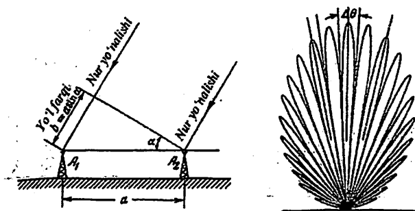
64-rasm. Radiointerferometrda nurlar yo'lining farqi va yo'naltirilganlik diagrammasi
