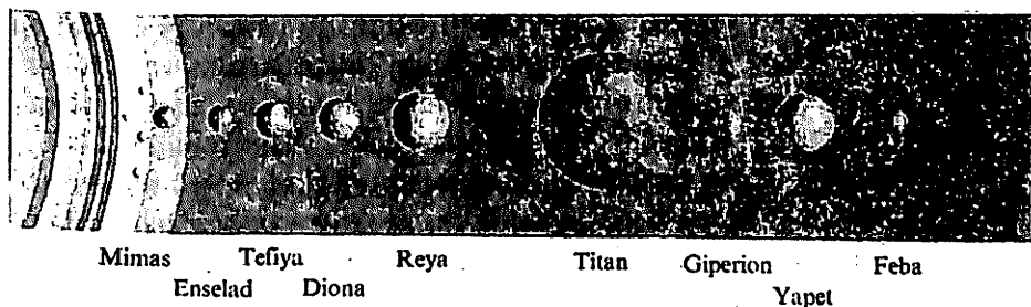
109-rasm. Saturnning yirik yo‘ldoshlari
