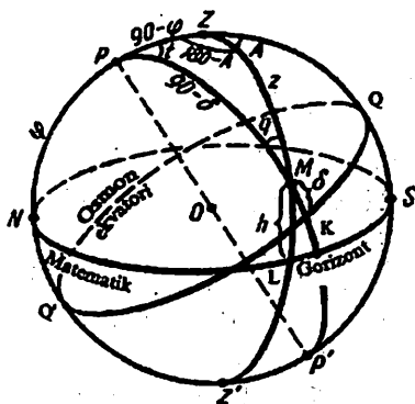
17-rasm. Parallaktik uchburchak va koordinatalarni almashtirish
