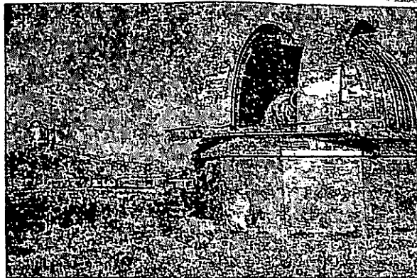
75-rasm. Toshkent astronomiya institutiga qarashli Maydanoq balantog' observatoriyasi
