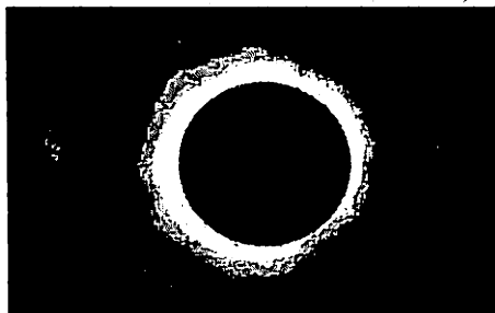
46-rasm. Quyoshning to'la tutilishi
