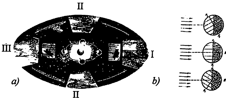
40-rasm. Sayyoramizda yil fasllarining kuzatilishi
