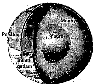
94-rasm. Veneraning ichki tuzilishi
