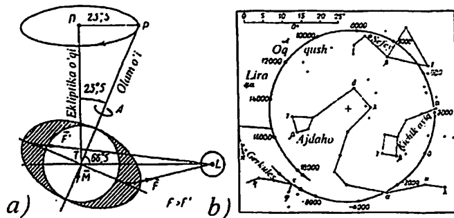
41-rasm. Pretsessiya hodisasini tushuntirish
