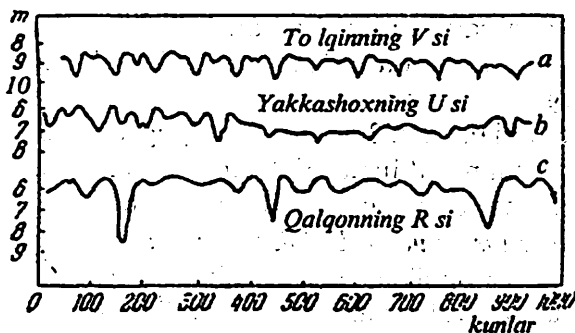
142-rasm. Savrning RV tipidagi yulduzlar ravshanligining o'zgarishi
