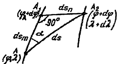
5-rasm. Elementar sferoidik uchburchak
