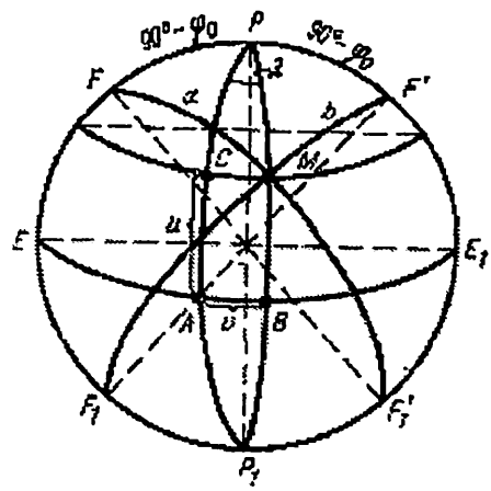
3-rasm. Elliptik koordinatalar tizimi
