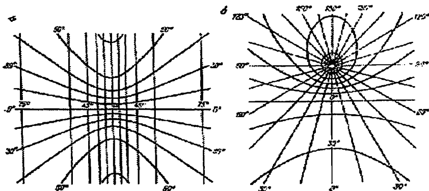
29-rasm. Gnomonik proyeksiyalar: a – ko'ndalang; b – qiyshiq
