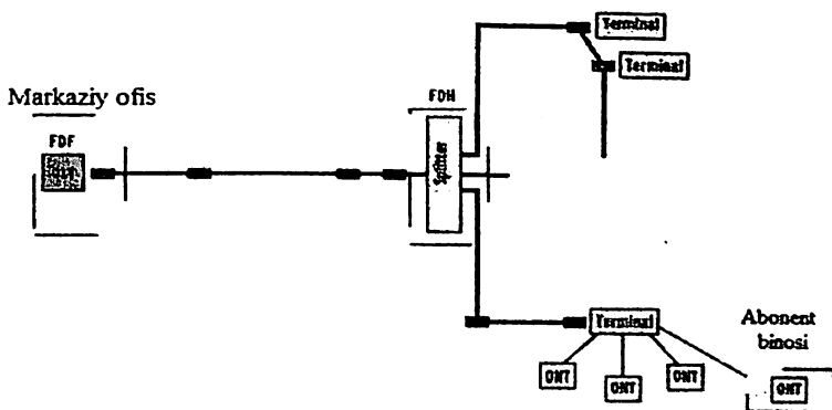
11.2-rasm. FTTx tarmog‘ida optik bog‘lanish
