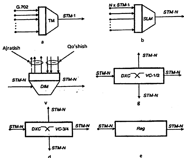
5.1 – rasm. TM (a,b), ADM (v), DXC(g,d) va regeneratlarning shartli (e) belgilanishlari
