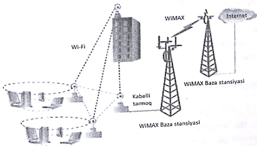
4.12-rasm. WMAN- Shahar simsiz tarmog'i
