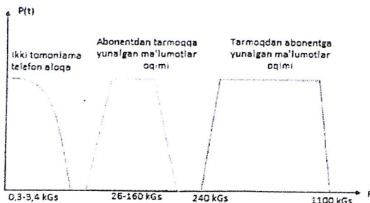
4.3- rasm. ADSL kanallariga chastotaning taqsimlanishi
