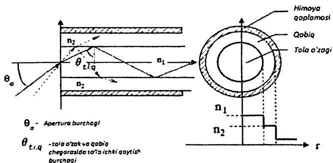
2.9-rasm. Optik toladan optik nurni tarqalish jarayoni
