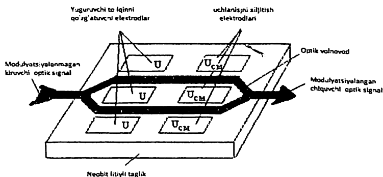
3.11-rasm. Max-Sender interferometri turidagi elektrooptik modulyatorning tuzilish sxemasi
