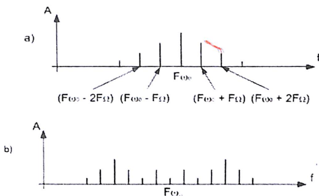
3.5-rasm. CHM signallaning spektrlari
