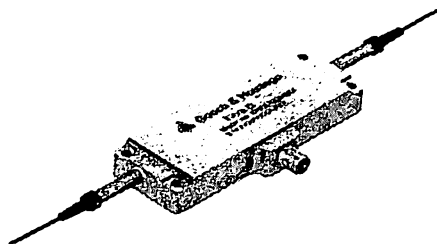
3.14-rasm. T-M110-0.2C2J-3-F2S seriyali akustooptik modulyator
