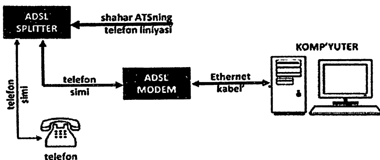
9.6-rasm. Abonent inshootida ADSL tarmog'ining oddiy ulanish sxemasi
