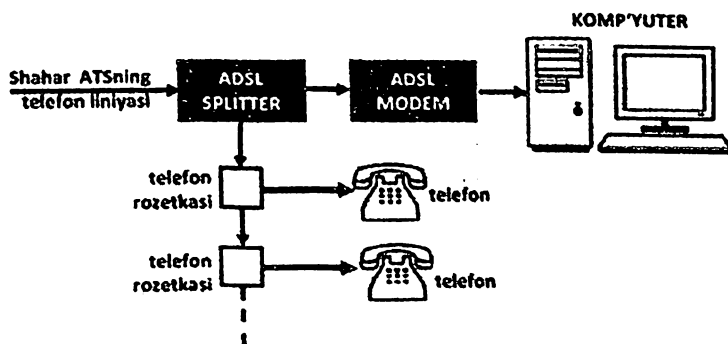
9.7-rasm. Abonent inshootida ADSL tarmog'iga ikki telefon apparatining ulanish sxemasi
