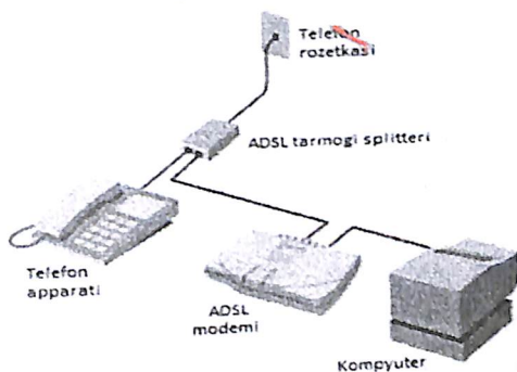
4.5-rasm. Abonent inshootida ADSL modem va uning komponentalarini ulanish ketma-ketligi
