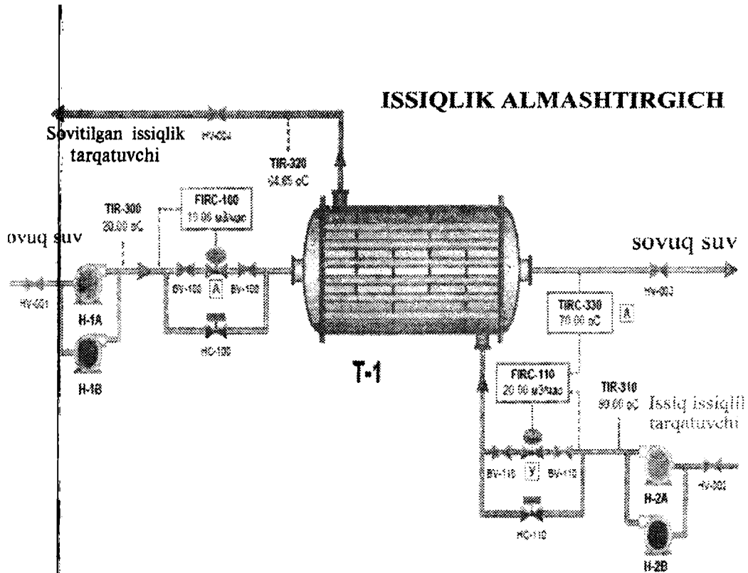
7.3-rasm. Isitish sxemasi.
