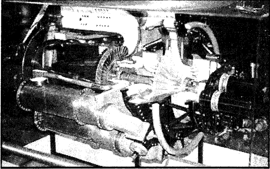
5.3-rasm. Radial markazdan qochma kompressor bilan prepatlangan TRD General Electric J-31.
