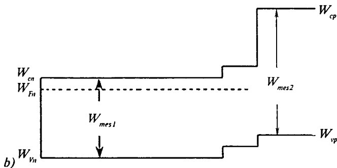
4.8-rasm. Geteroo'tishli fotodiodning tuzilishi (a) va energetik diagrammasi (b)
