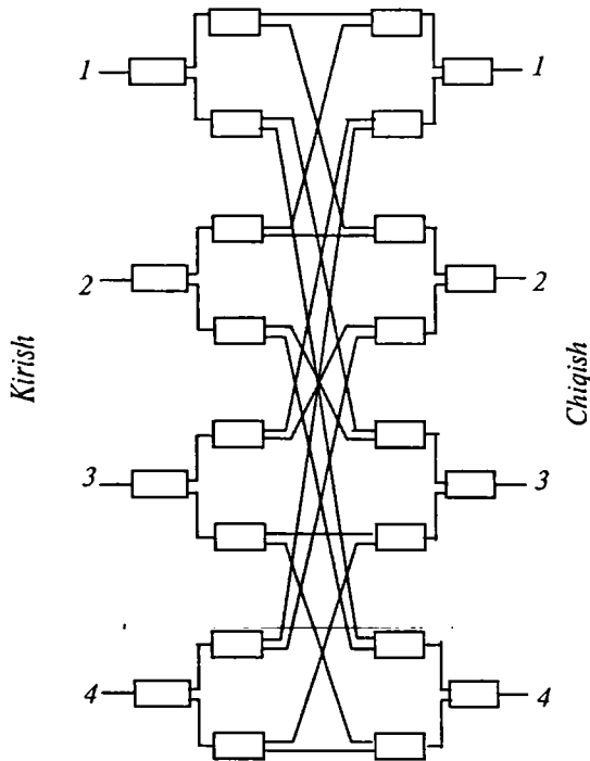
10.9-rasm. Shpenkening KSS sxemasi
