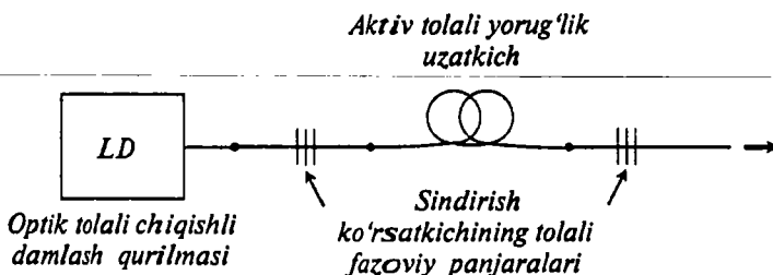
14.6-rasm. Tolali lazerning tuzilishi
