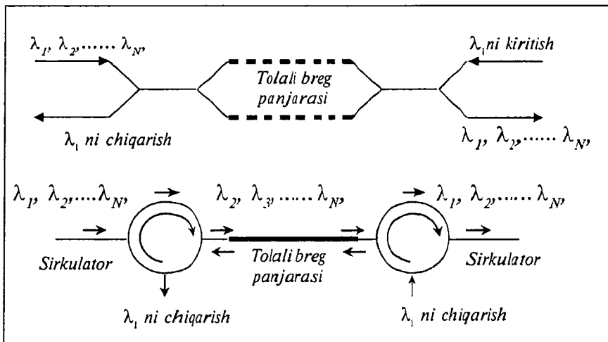
9.7-rasm. Tolali breg panjarasidan kanallarni kiritish va chiqarish uchun foydalanish
