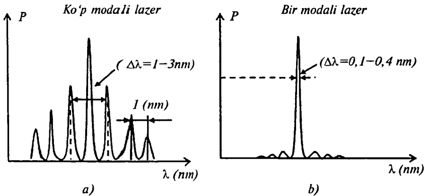
3.22-rasm. Lazer diodlarning nurlanish spektrlari: a – ko'p modal laser diodining nurlanish spektri; b – bir modal laser diodining nurlanish spektri
