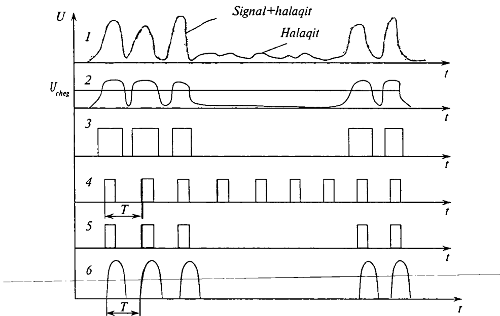
11.3-rasm. Regeneratorsining vaqt diagrammasi
