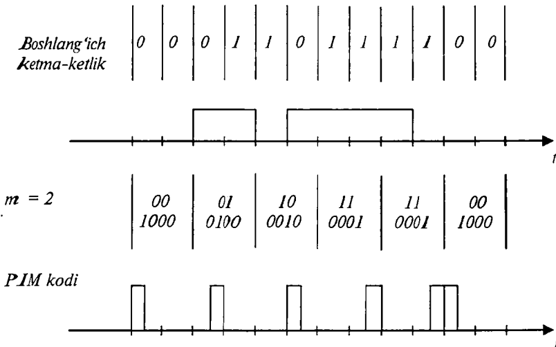
11.8-rasm. PIM kodining shakllanishi
