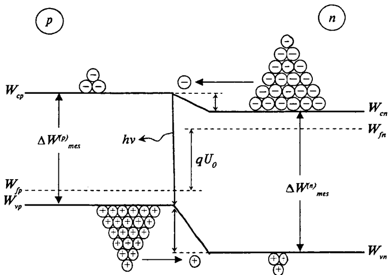
3.9-rasm. Getero tuzilishli yorug‘lik diodining energetik diagrammasi
