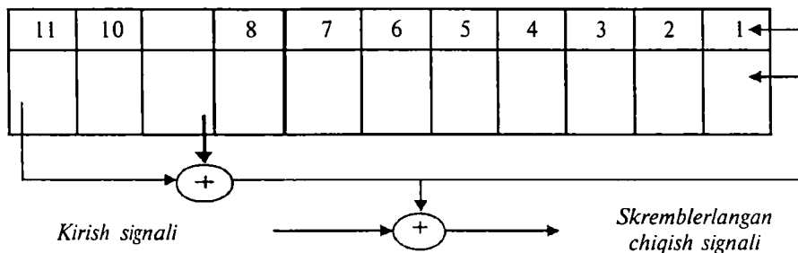
11.10-rasm. Skremblerlash qurilmasining ishi
