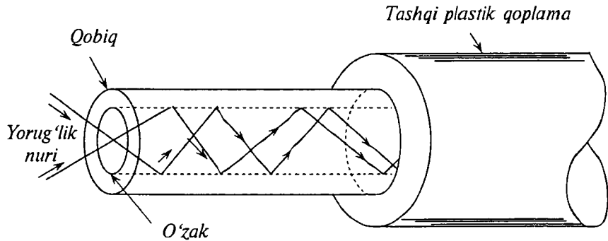
2.2-rasm. Optik tolaning tuzilishi
