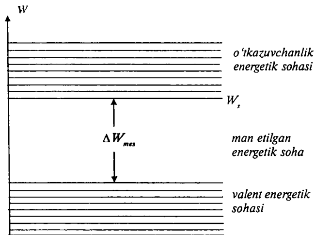
3.11-rasm. Yarimo'tkazgichning energetik diagrammasi
