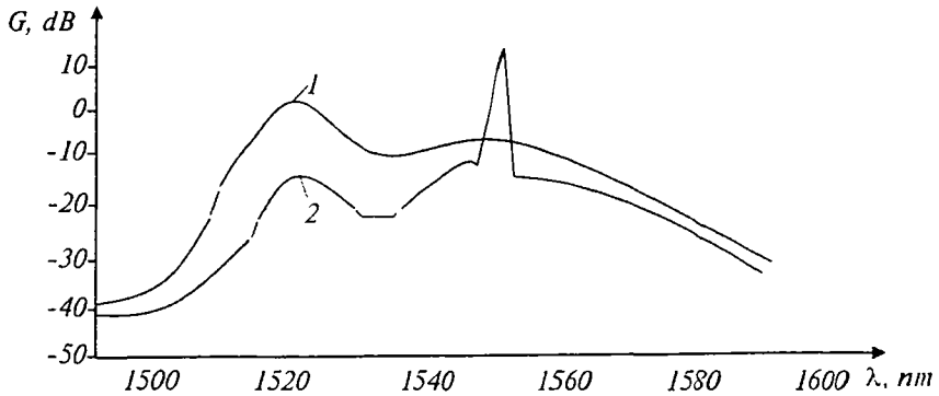
5.9-rasm. Totali optik kuchaytirgichning chiqish nurlanish spektri:
