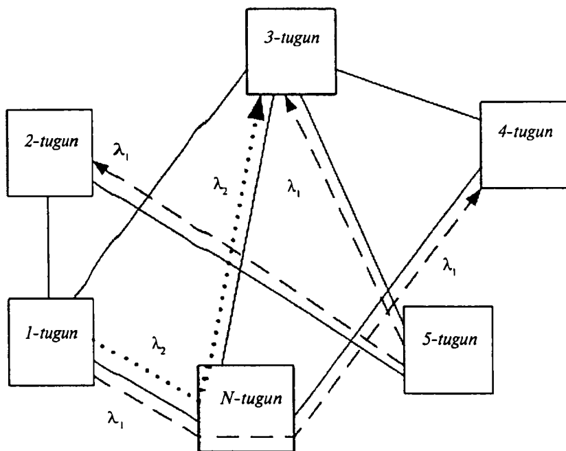
12.3-rasm. Passiv to‘lqin marshrutlashtirishli optik tarmoq
