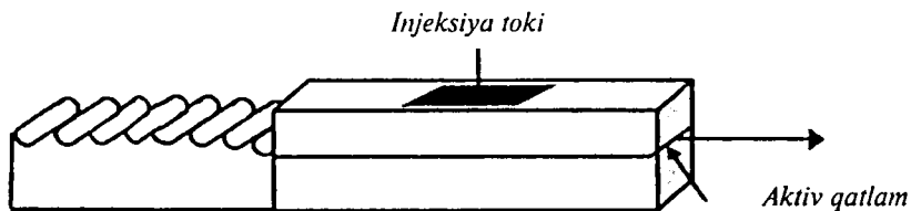
3.24-rasm. Taqsimlangan Bregg ko'zguli lazer diodi
