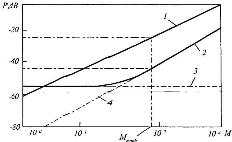
6.14-rasm. Signal (1), issiqlik (3), drob (4) va yig'indi shovqinlarining kuchayish koeffitsiyentiga bog'liqligi
