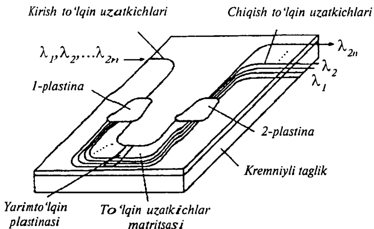
9.5-rasm. Tolali optik multipleksorning tuzilishi
