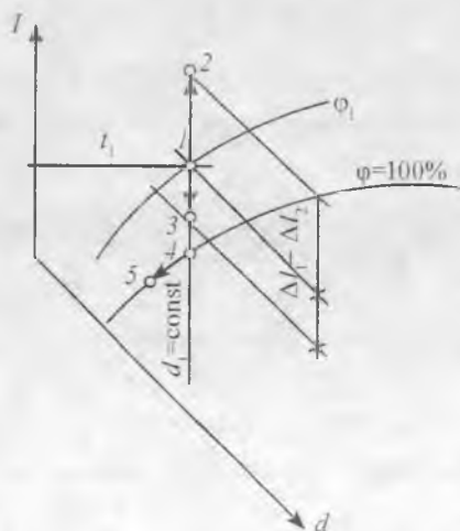
44-rasm. Isitish va sovitish jarayonlari ko'rsatilgan h-d diagrammasi: 1 – havoning boshlang'ich holati; 2 – havoning oxirgi holati; 1-2 – havoning holati o'zgarish jarayoni.
