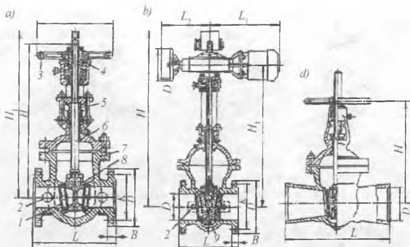
14-rasm. So'riluvchan shpindelli po'lat ponasimon zulfar:
