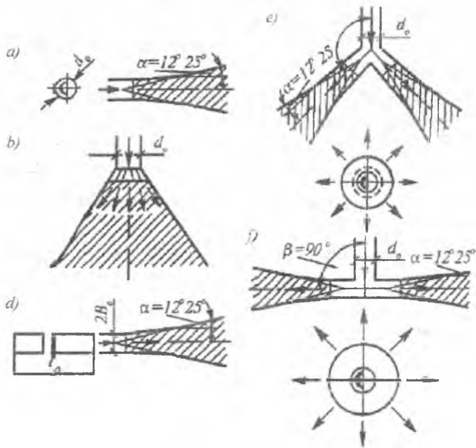
32-rasm. Turli shakldagi oqimlar:
