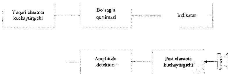
10.4-rasm. Elektromagnit nurlanish indikatorining sxemasi.
