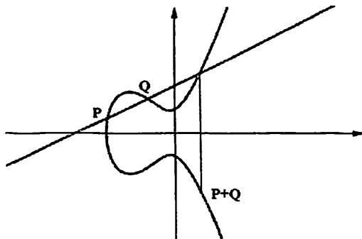
1.8-rasm. Nuqtalarni qo'shishning geometrik ifodalanihi
