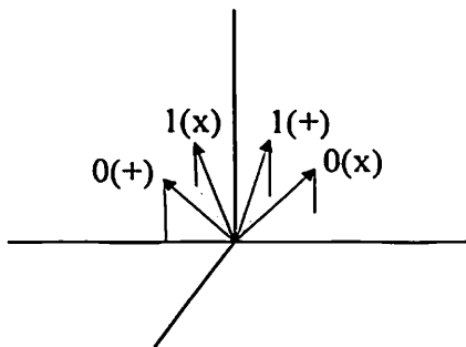
8.10-rasm. BB84(4+2) prtokolida qo'llaniladigan polyarizasiya holati
