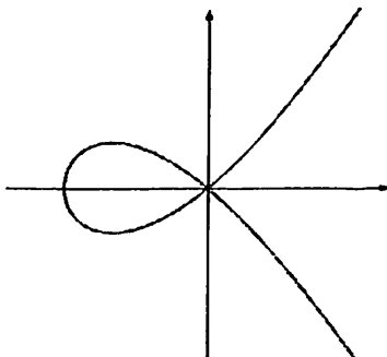
1.2-rasm. y^2 = x^3 + x^2 elliptik egri chiziq grafigi
