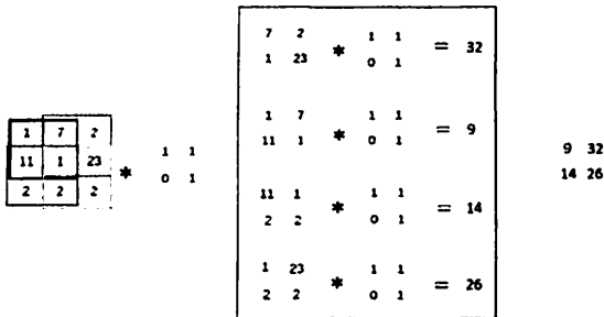
4.2.8-rasm. Feture Maps hisoblash jarayoni
