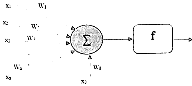
4.1.4-rasm. Eng sodda neyron modeli
