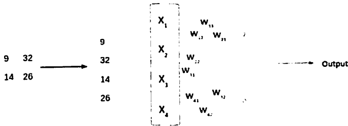
4.2.10-rasm. Neyron qatlamini hisoblash(Full connekt)
