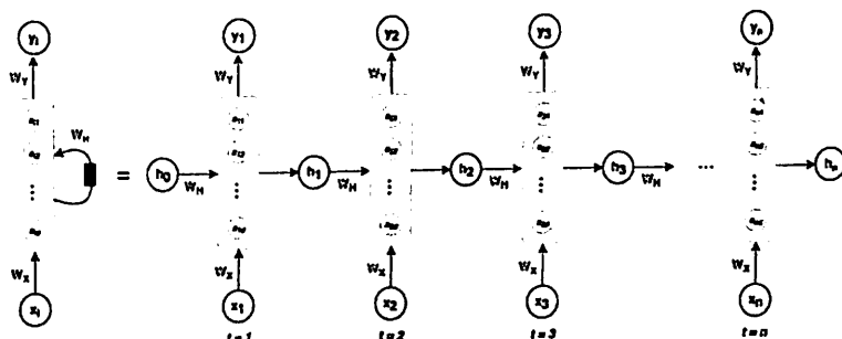
4.2.14-rasm. Recurrent neyron tarmoq
