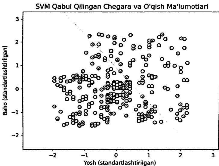
3.2.15-rasm. SVM algoritmi asosida sinflashtirish
