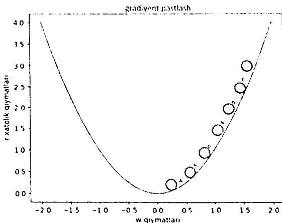
3.1.5– rasm. Gradiyent pastlash grafigasi
