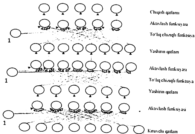
4.1.5-rasm.Uchtalik chuqurlikka ega oldinga harakatlanuvchi neyron tarmoq
