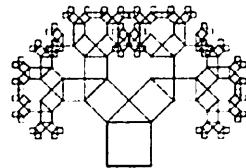
n=6, \alpha=\pi/4
