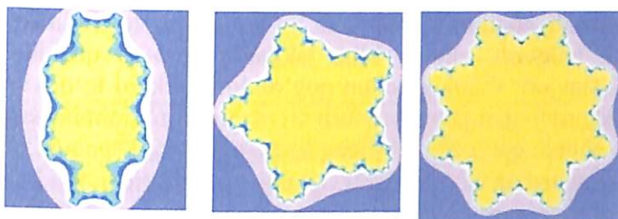
2.10-rasm. Mandelbrot fraktal naqshi
