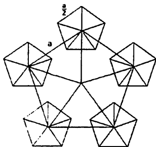
4.6-rasm. Beshburchakli fraktallar, 1-qadam va 2-qadamda
