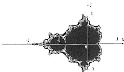
3.8-rasm. Mandelbrot to'plami
