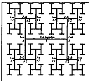
3.13-rasm. 6-tartibdagi "Keyli daraxti"
