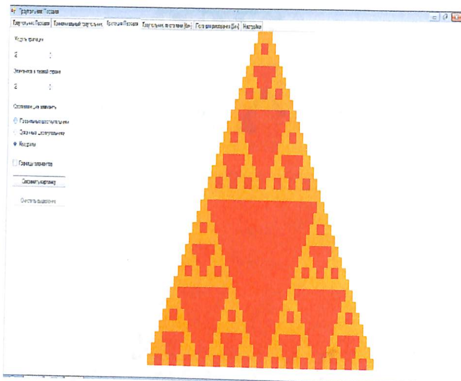
5.29-rasm. Paskal Trapezoid yorlig‘i
