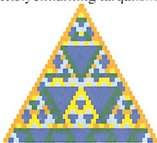
5-33-rasm. Paskal uchburchagi modulida binomial koeffitsiyentlarning tarqalishi
