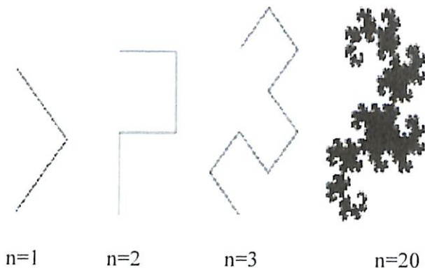
2.9-rasm. Ajdaho egri chizig‘i
