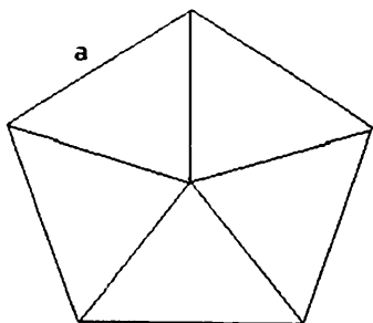
4.6-rasm. Beshburchakli fraktallar, 1-qadam va 2-qadamda
