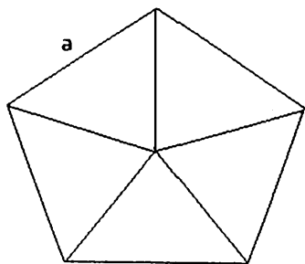
4.7-rasm. Beshburchakli fraktallar, 1-qadam va 2-qadamda
