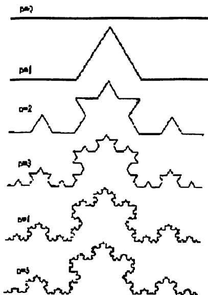
1.2-rasm. n=1, \dots, 5 larda Kox triad egri chizig‘ini qurish
