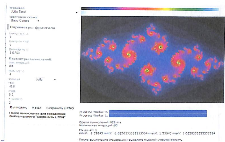
2.7-rasm. Dasturda Julia to‘plamlarini qurish
