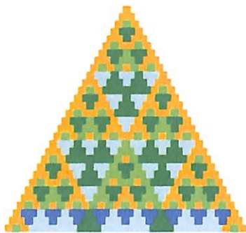
5.34-rasm. Paskal uchburchagidagi binomial koeffitsiyentlarining n=3 darajadagi tarqalishi
