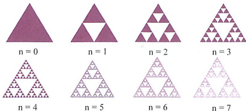
3.12-rasm. Serpin salftkasi
