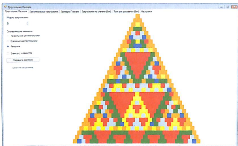
5.25-rasm. Tanlangan qiymat moduli 6 bo‘lgan “Paskal uchburchagi”.
