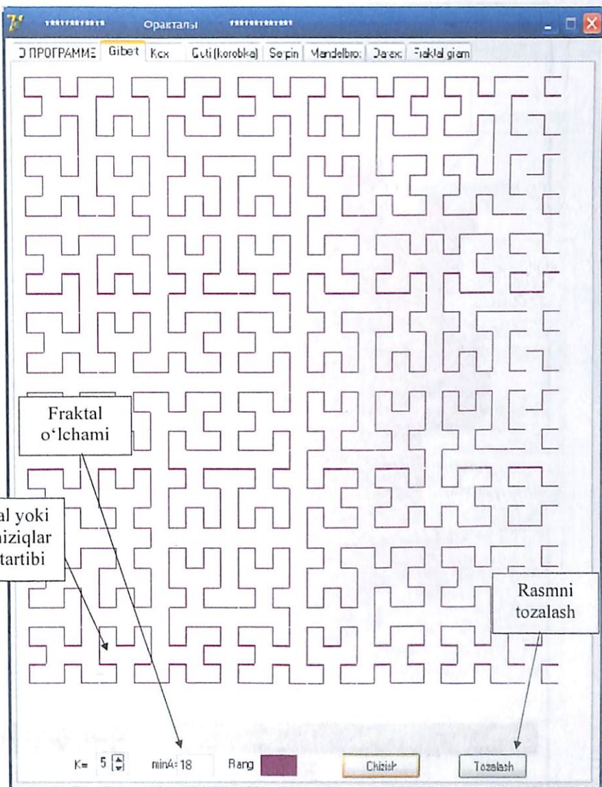
5.14-rasm. Gilbert egri chizig'i
