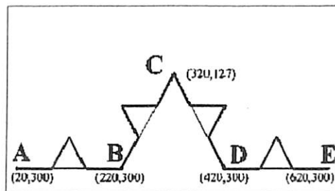
3.6-rasm. IFS usulida Kox triad egri chizig'i qurish uchun tayyorgarlik
