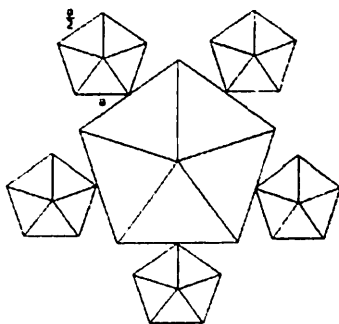
4.7-rasm. Beshburchakli fraktallar, 1-qadam va 2-qadamda
