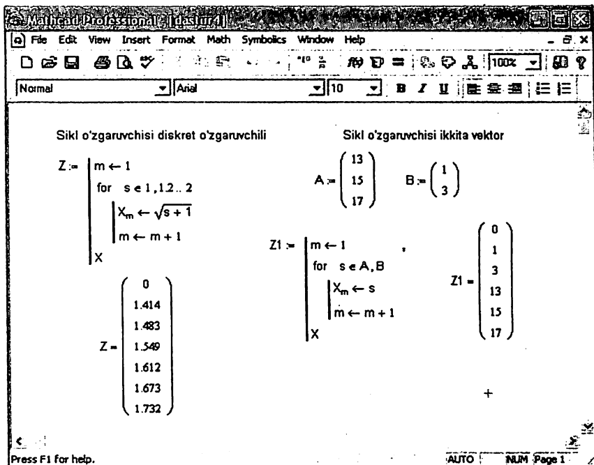
3.24.-rasm. Dasturlashda For sikl operatorini qo'llash.
