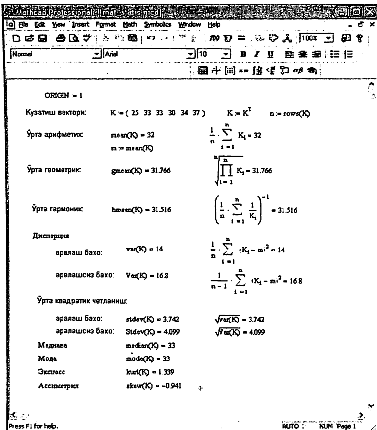
3.19.-rasm.Statistika kattaliklarini hisoblash.
