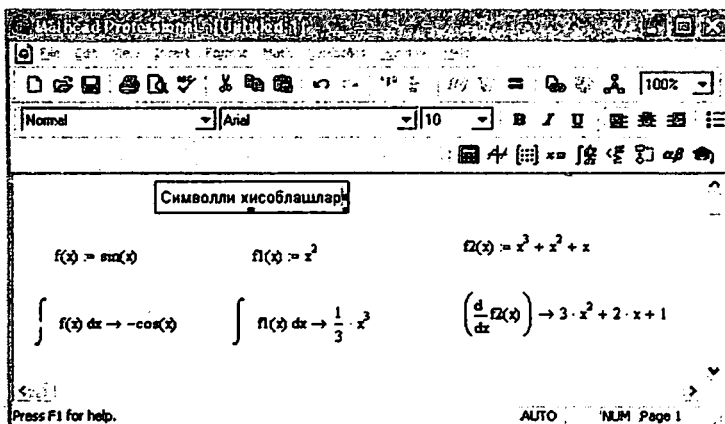
3.6.-rasm. Simvolli hisoblashlarni bajarish.
