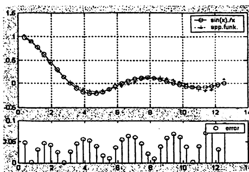
2.27-rasm. Grafik ko'rinishi
