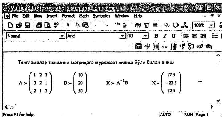
3.15.-rasm. Tenglamalar tizimini matritsa usulida yechish.
