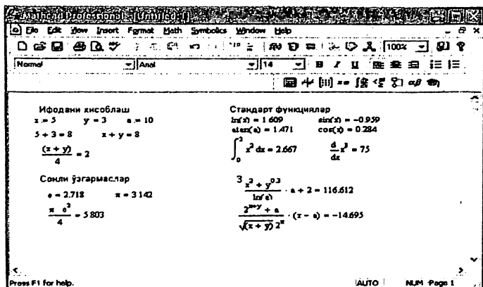
3.2-rasm. Oddiy matematik ifodalarni hisoblash.
