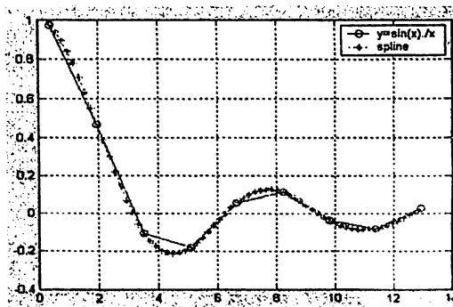
2.29-rasm. Kubik ko'phad.
