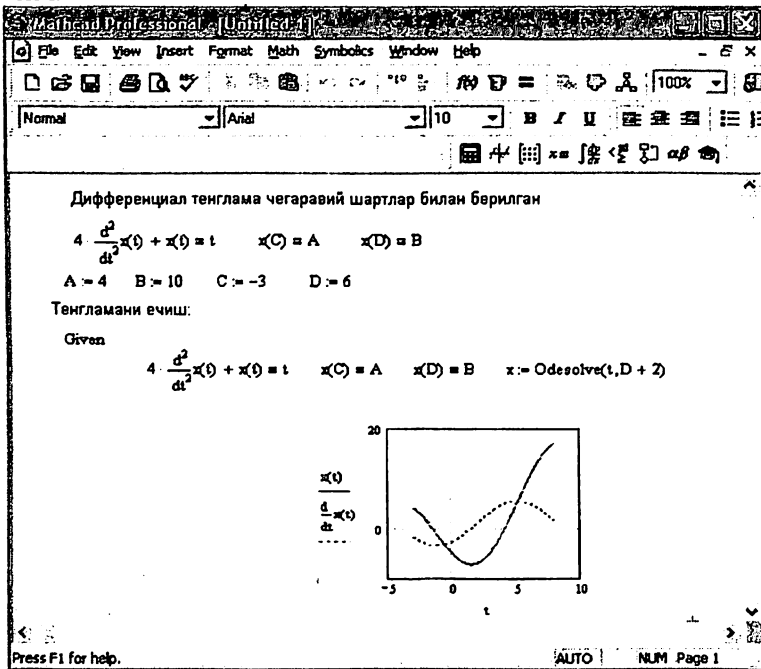
3.16.-rasm. Differensial tenglamalarni yechish.
