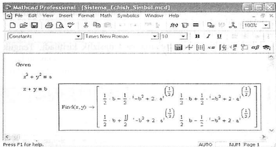
7.15-rasm. Chiziqsiz tenglamalar tizimini simvoli yechimini topish
