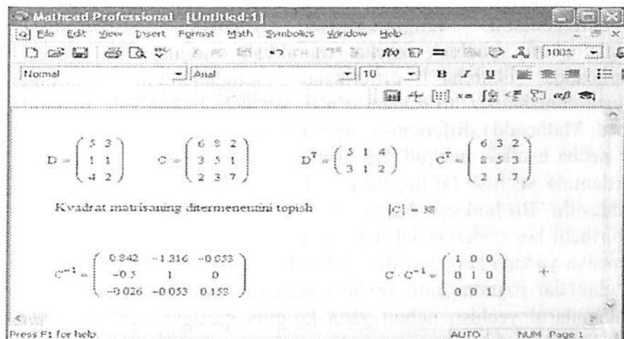
7.17-rasm. Matritsa ustida amallar bajarish
