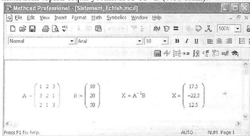
7.18-rasm. Tenglamalar tizimini matritsa usulida yechish
