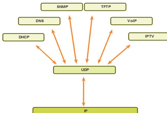
4.9 – rasm. TCP va UDP protokollar foydalanadigan ilovalari
