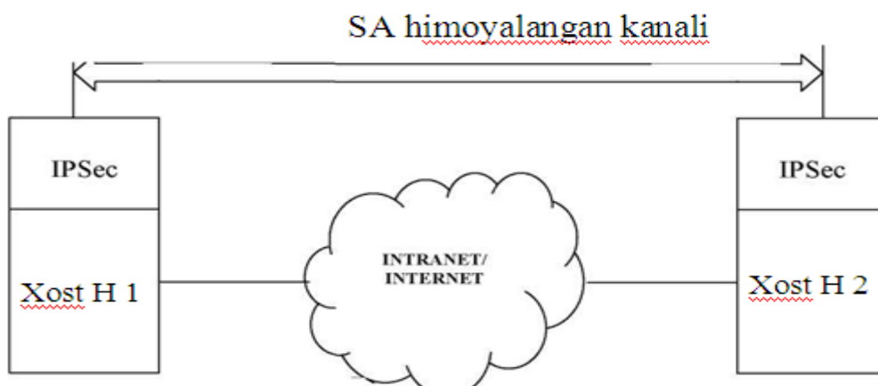
5.9 - rasm. "Xost-xost" sxemasi
