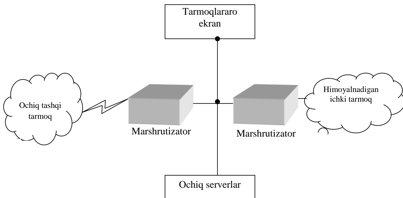
8.11- rasm. Bitta tarmoq interfeysli firewall yordamida lokal tarmoqni himoyalash
