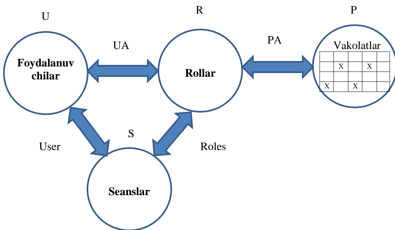
4.1-rasm. Foydalanishni boshqarishning rolli modeli
