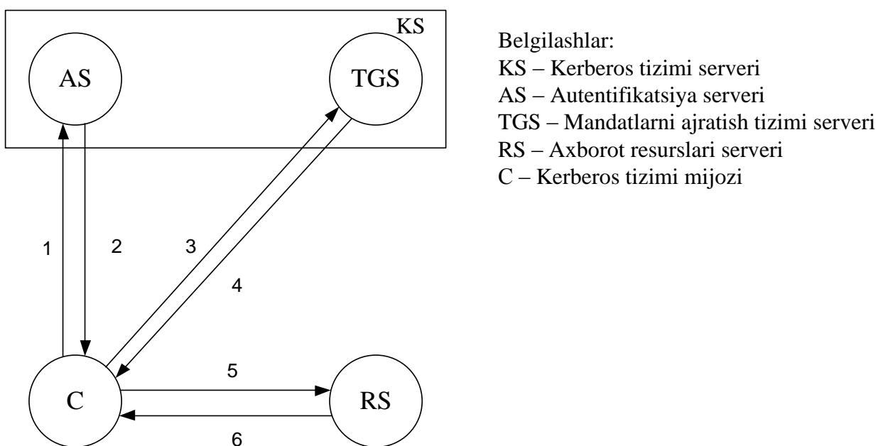
6.2-rasm. Kerberos protokolining ishlash sxemasi
