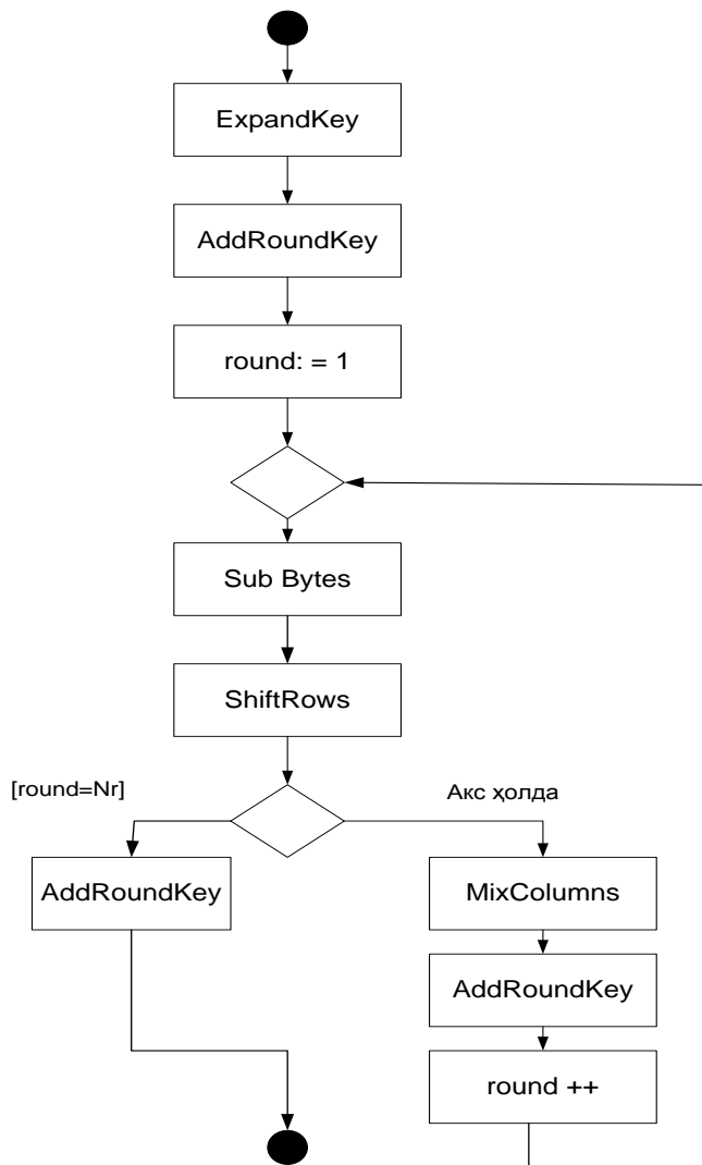
5.12-rasm. Shifrlash jarayoni
