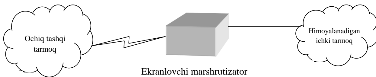
8.10-rasm. Tarmoqlararo ekran – ekranlovchi marshrutizator
