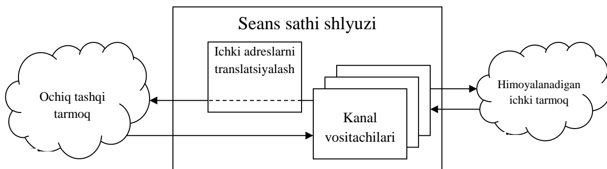
8.8-rasm. Seans sathi shlyuzining ishlash sxemasi
