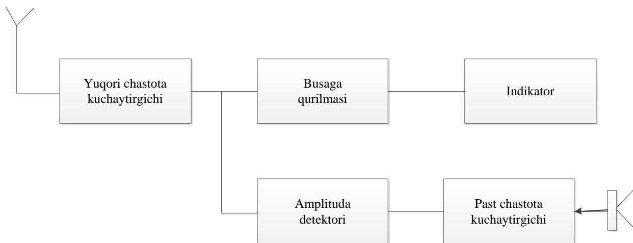
10.4-rasm. Elektromagnit nurlanish indikatorining sxemasi
