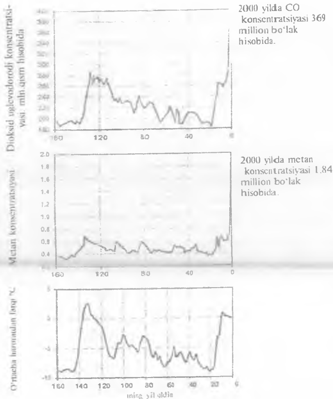
8-rasm. Parnik gazi va o'rtacha global harorat o'tgan 160 ming yilda.
