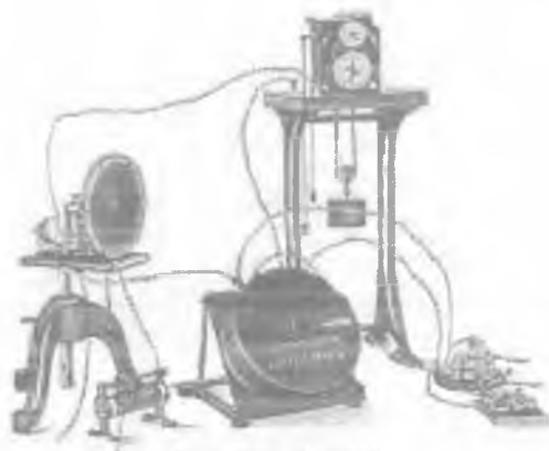
1- rasm. Xronoskop.
