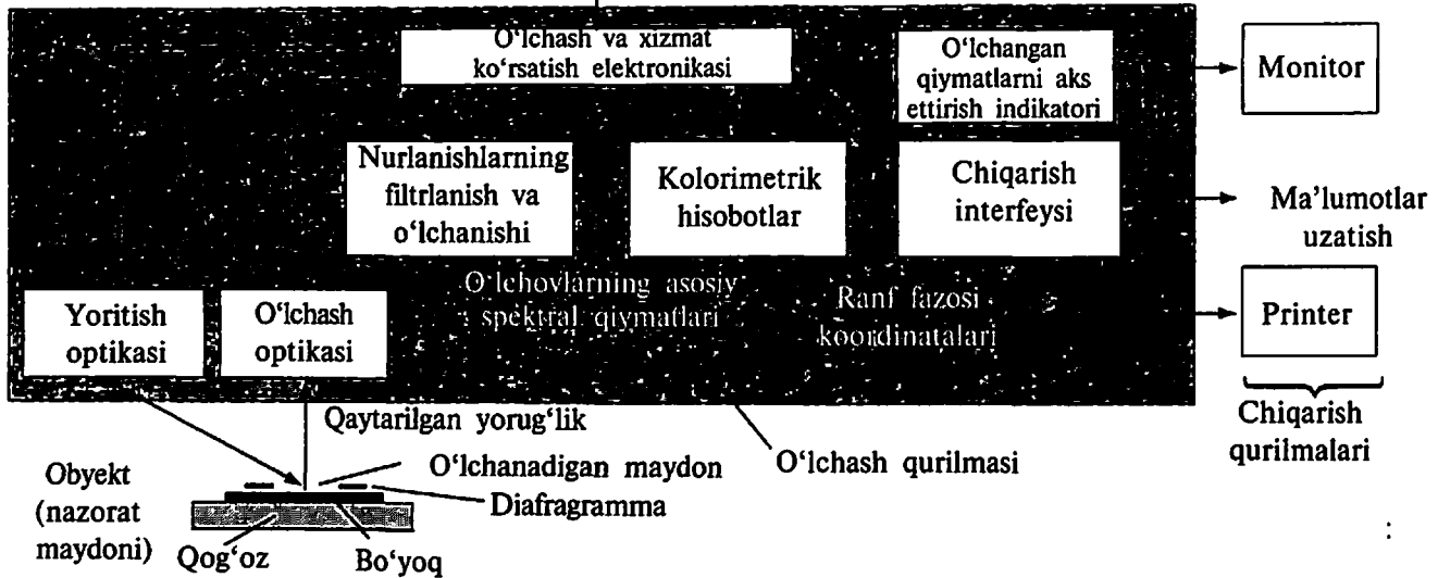
12.8-rasm. Rangni o'lchash moslamasi tuzilishining blok-sxemasi
