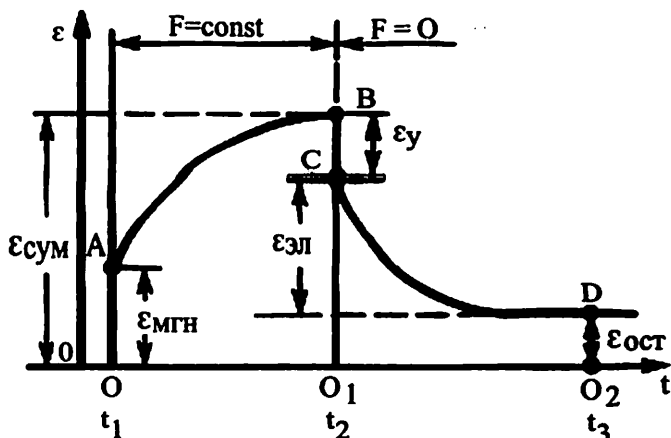
4.5-rasm. O'zgarmas kuch ta'sirida dekelning deformatsiyaning o'sishi
