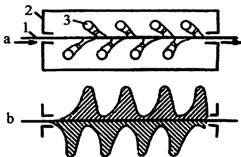
6.2-rasm. Gaz alangasida matoga ishlov berish prinsipi: a) issiqlik berish tizmasi; b) issiqlikni taqsimlanish tizmasi
