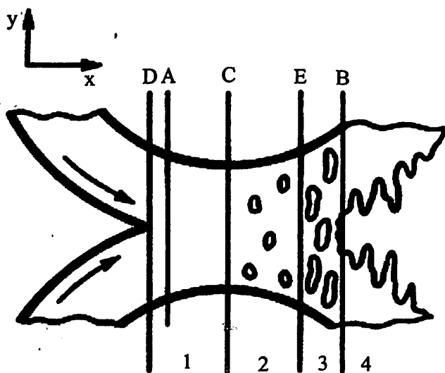
3.6-rasm. Bo‘yoq qatlamining parchalanish mexanizmi tizmasi
