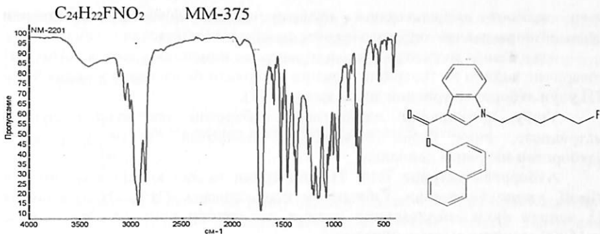
4.3 расм. NM-2201 Naphthalen-1-yl-1-(5-fluoropentyl)-1H-indole-3-carboxylate ning ИК спектри
