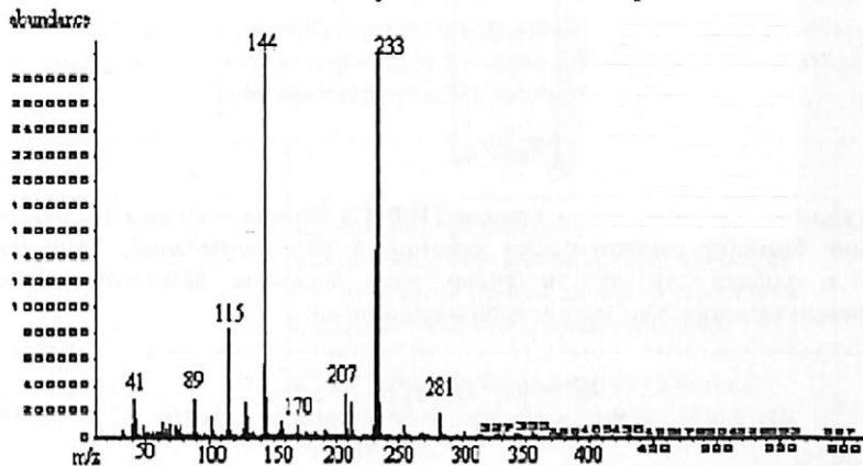
4.4 расм. NM-2201 Naphthalen-1-yl-1-(5-fluoropentyl)-1H-indole-3-carboxylate ning ГХ-МС таҳлили
