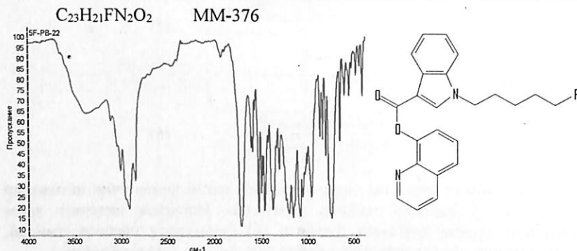
4.1 расм. 5Fluoro-PB-22 Quinolin-8-yl 1-pentyfluoro-1H-indole-3-8-carboxylate нинг ИК спектри
