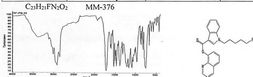
Рис. 2.4.1. ИК спектры 5Fluoro-PB-22 Quinolin-8-yl 1-pentyfluoro-1H-indole-3-8-carboxylate
