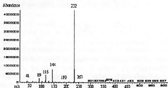
Рис. 2.4.2. Масс спектры 5Fluoro-PB-22 Quinolin-8-yl 1-pentyfluoro-1H-indole-3-8-carboxylate
