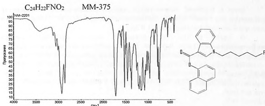
Рис. 2.4.3. ИК- спектры NM-2201 Naphthalen-1-yl-1-(5-fluoropentyl)-1H-indole-3-carboxylate
