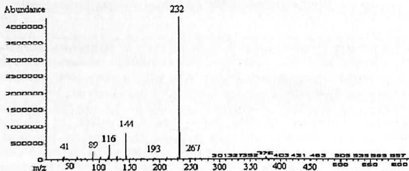
4.2 расм. 5Fluoro-PB-22 Quinolin-8-yl 1-pentyfluoro-1H-indole-3-8-carboxylate нинг ГХ-МС таҳлили
