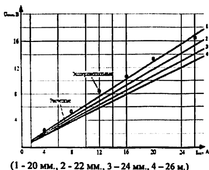
Fig.6 Steady-state features of output voltage under different FMW under importances of the air clearance ( points - an experiment, line - a design values)
