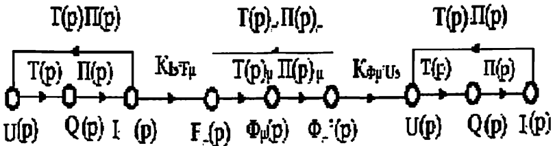
Fig. 3. The Dinamic graphs model of the electromagnetic transducers current to voltage
