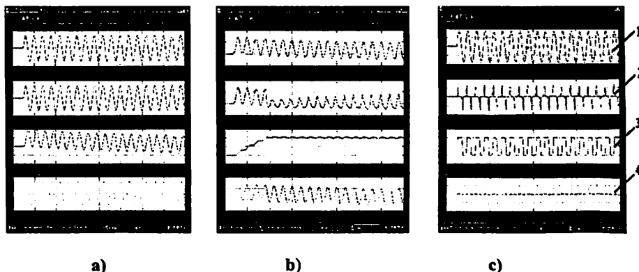
Fig.5. Graphics of input (1 - a primary current - I_e in), intermediate (2 - m.m.p. F1 and 3- magnetic flow - F2) and output (4 - a secondary voltage U_e out) of the values of the electromagnetic transducers of the current to voltage under: normal (a), asymmetrical (b) mode and in mode of the short circuit (c) in electric networks of energy system
