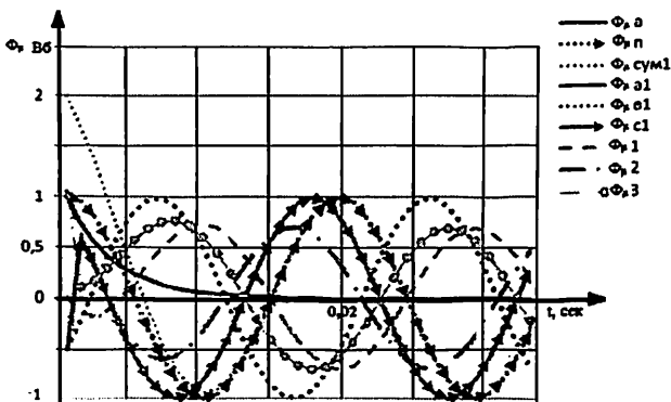
Fig.10. Graphics of magnetic flows in magnetic system of the electromagnetic transducers of the current to voltage with flat measure winding during flow primary current on three-phases electrical networks of energy systems
