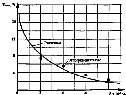
Fig.7. Dependency of the U out with different importances
