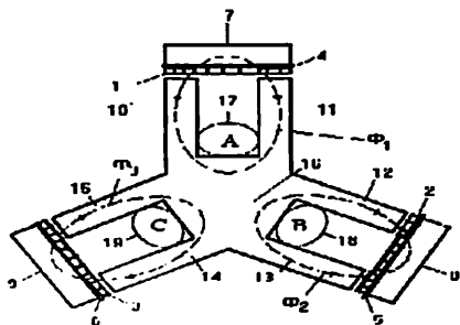
1, 2, and 3 – FMW, 4, 5 and 6 – insulation plastins, 7,8 and 9 – additional Cores, 10 and 11, 12 and 13. 14 and 15 – pairs if parallel cterjens,16– base of core, 17, 18 and 19– primary windings
