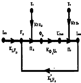
Fig.11. Graph model for research of the sources of inaccuracy output voltage U_{cout}
