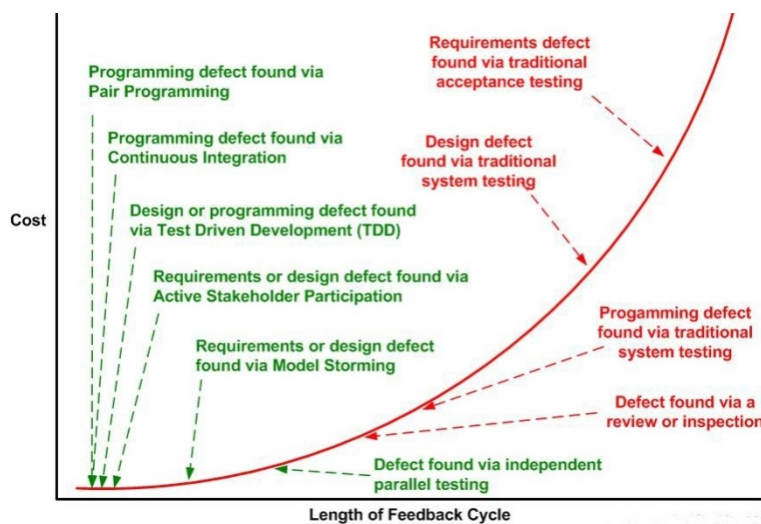
Figure 14: Comparison of Feedback cycles with traditional approaches. (Source: http://www.ambysoft.com )
