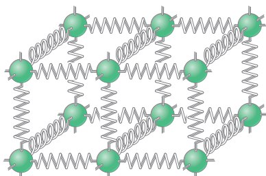
FIGURE D-5 The atoms in a crystalline solid can vibrate about their equilibrium positions as if they were connected to their neighbors by springs. (The forces between atoms are actually electrical in nature.)
