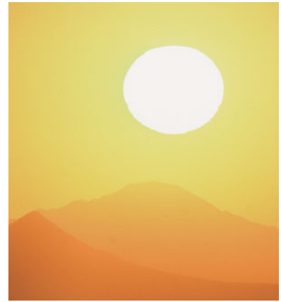
FIGURE 14–10 The Sun’s surface radiates at 6000 K—much higher than the Earth’s surface.
