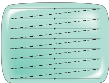
FIGURE 17–30 Electron beam sweeps across a CRT television screen in a succession of horizontal lines. Each horizontal sweep is made by varying the voltage on the horizontal deflection plates (Fig. 17–29). Then the electron beam is moved down a short distance by a change in voltage on the vertical deflection plates, and the process (referred to as a raster) is repeated.
