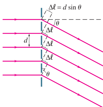
FIGURE 24-24 Diffraction grating.
