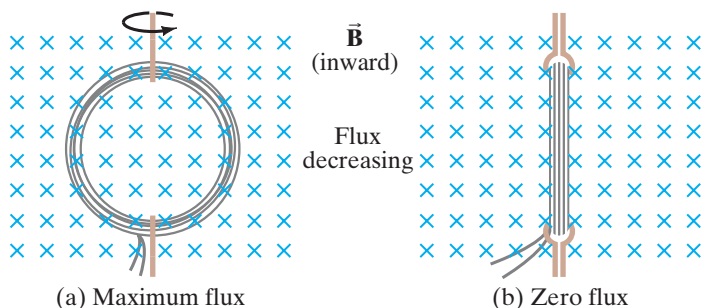
FIGURE 21–6 A current can be induced by rotating a coil in a magnetic field. The flux through the coil changes from (a) to (b) because \theta (in Eq. 21–1, \Phi = BA \cos \theta ) went from 0^\circ ( \cos \theta = 1 ) to 90^\circ ( \cos \theta = 0 ).
