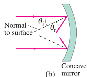
FIGURE 23-10 Mirrors with convex and concave spherical surfaces. Note that \theta_r = \theta_i for each ray. (The dashed lines are perpendicular to the mirror surface at each point shown.)
