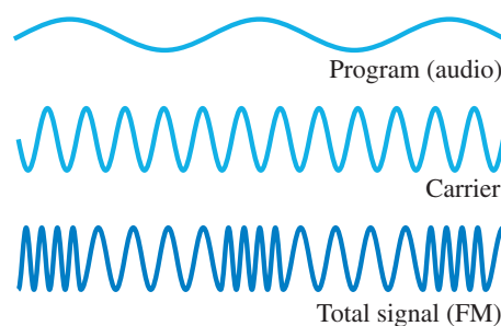
FIGURE 22–15 In frequency modulation (FM), the frequency of the carrier signal is made to change in proportion to the audio signal’s amplitude. This method is used by FM radio and television.
