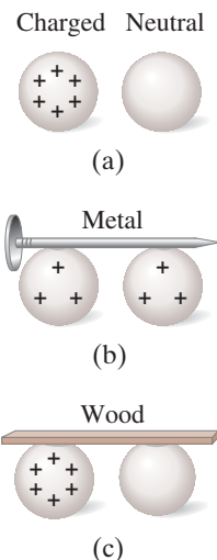
FIGURE 16-5 (a) A charged metal sphere and a neutral metal sphere. (b) The two spheres connected by a conductor (a metal nail), which conducts charge from one sphere to the other. (c) The original two spheres connected by an insulator (wood); almost no charge is conducted.
