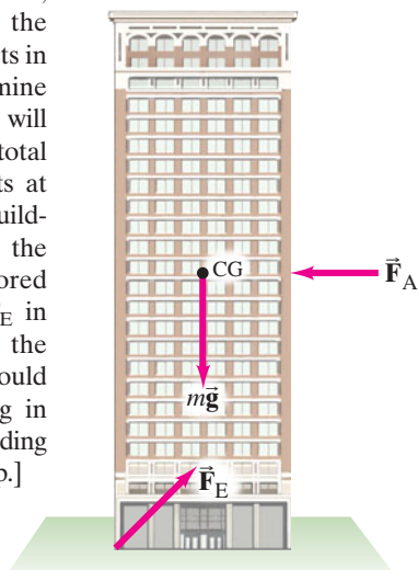
FIGURE 9–80 Forces on a building subjected to wind ( \vec{F}_A ), gravity ( m\vec{g} ), and the force \vec{F}_E on the building due to the Earth if the building were just about to tip. Problem 61.
