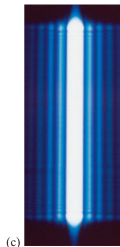
FIGURE 24-19 Diffraction pattern of (a) a circular disk (a coin), (b) scissors, (c) a single slit, each illuminated by a (nearly) point source of coherent monochromatic light.
