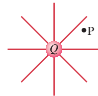
FIGURE 16-22 An electric field surrounds every charge. The red lines indicate the electric field extending out from charge Q , and P is an arbitrary point.
