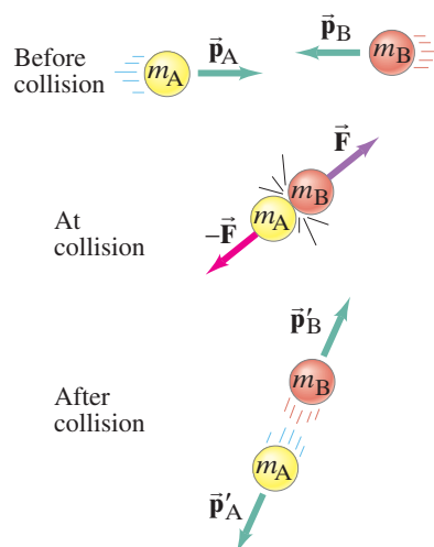
FIGURE 7-4 Collision of two objects. Their momenta before collision are \vec{p}_A and \vec{p}_B , and after collision are \vec{p}'_A and \vec{p}'_B . At any moment during the collision each exerts a force on the other of equal magnitude but opposite direction.
