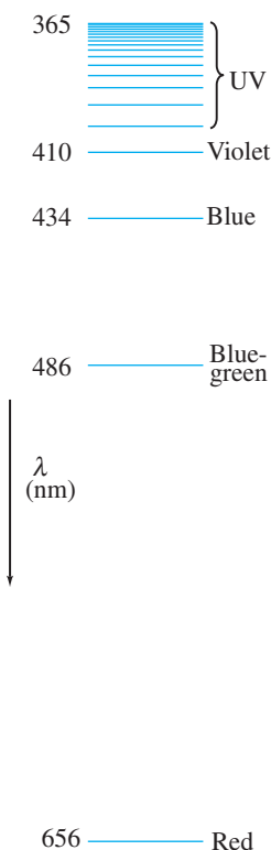
FIGURE 27-24 Balmer series of lines for hydrogen.
