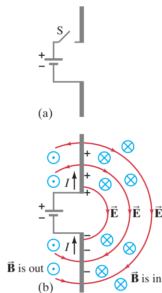
FIGURE 22–4 Fields produced by charge flowing into conductors. It takes time for the \vec{E} and \vec{B} fields to travel outward to distant points. The fields are shown to the right of the antenna, but they move out in all directions, symmetrically about the (vertical) antenna.
