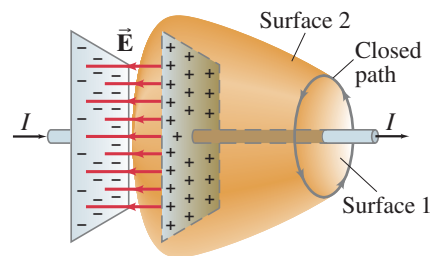
FIGURE 22–3 A capacitor discharging. A conduction current passes through surface 1, but no conduction current passes through the sacklike surface 2. An extra term is needed in Ampère’s law.
