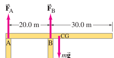
FIGURE 9–9 A cantilever.
