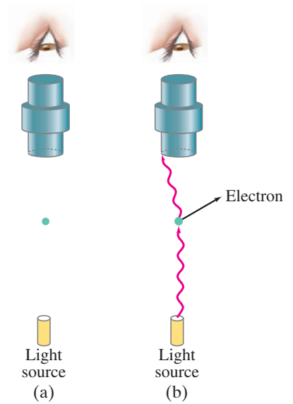
FIGURE 28–5 Thought experiment for observing an electron with a powerful light microscope. At least one photon must scatter from the electron (transferring some momentum to it) and enter the microscope.
