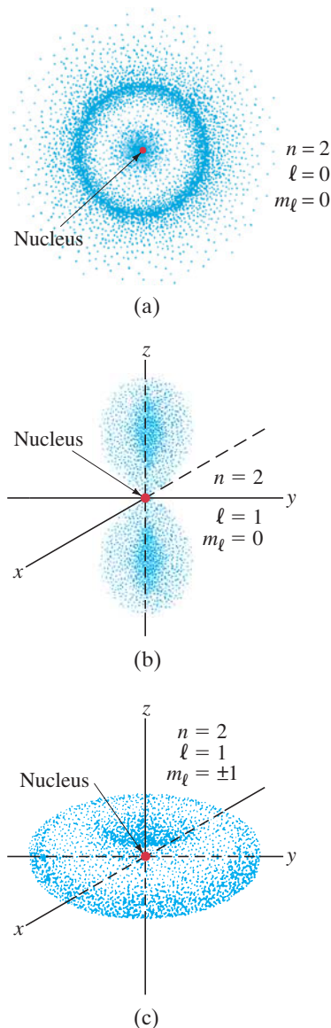
FIGURE 28-9 Electron cloud, or probability distribution, for n = 2 states in hydrogen. [The donut-shaped orbit in (c) is the sum of two dumbbell-shaped orbits, as in (b), along the x and y axes added together.]
