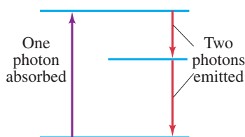
FIGURE 28–14 Fluorescence.
