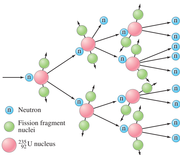
FIGURE 31–5 Chain reaction.
