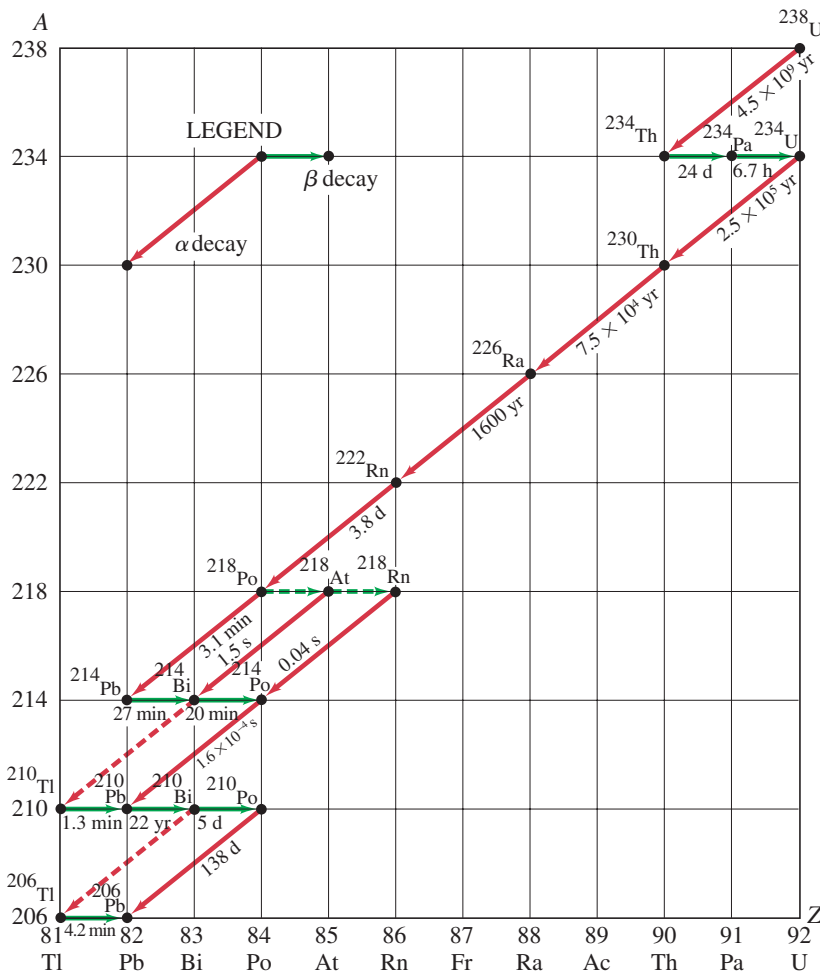
FIGURE 30-11 Decay series beginning with {}^{238}_{92}\text{U} . Nuclei in the series are specified by a dot representing A and Z values. Half-lives are given in seconds (s), minutes (min), hours (h), days (d), or years (yr). Note that a horizontal arrow represents \beta decay ( A does not change), whereas a diagonal line represents \alpha decay ( A changes by 4, Z changes by 2). For the four nuclides shown that can decay by both \alpha and \beta decay, the more prominent decay (in these four cases, >99.9\% ) is shown as a solid arrow and the less common decay ( <0.1\% ) as a dashed arrow.
