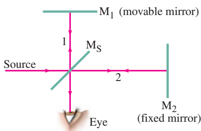
FIGURE 24–37 Michelson interferometer.
