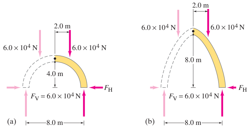
FIGURE 9–31 (a) Forces in a round arch, compared (b) with those in a pointed arch.
