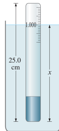
FIGURE 10–16 A hydrometer. Example 10–9.
