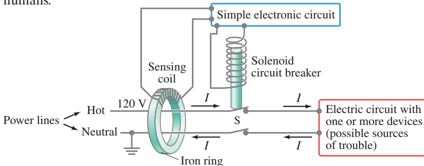
FIGURE 21-33 A ground fault circuit interrupter (GFCI).
