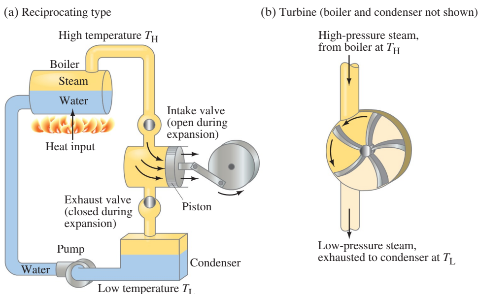
FIGURE 15–12 Steam engines.
