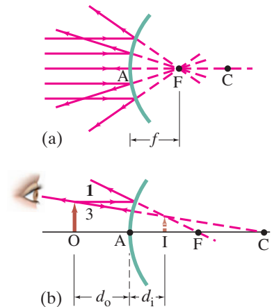
FIGURE 23–19 Convex mirror: (a) the focal point is at F, behind the mirror; (b) the image I of the object at O is virtual, upright, and smaller than the object. [Not to scale for Example 23–7.]
