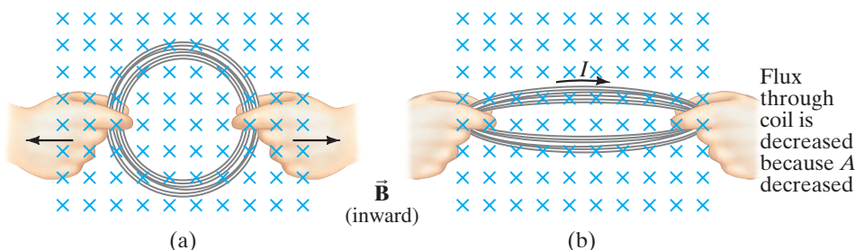
FIGURE 21–5 A current can be induced by changing the coil's area, even though B doesn't change. Here the area A is reduced by pulling on the sides of the coil: the flux through the coil is reduced as we go from (a) to (b). The brief induced current acts in the direction shown so as to try to maintain the original flux ( \Phi = BA ) by producing its own magnetic field into the page. That is, as area A decreases, the current acts to increase B in the original (inward) direction.
