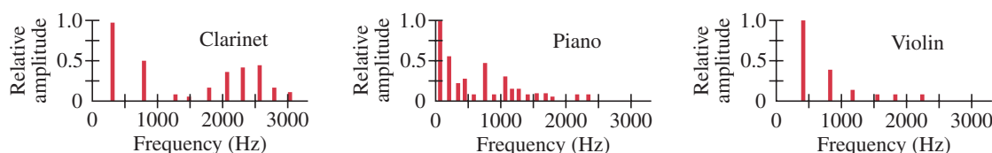
FIGURE 12–15 Sound spectra for different instruments. The spectra change when the instruments play different notes. The clarinet is a bit complicated: it acts like a closed tube at lower frequencies, having only odd harmonics, but at higher frequencies all harmonics occur as for an open tube.
