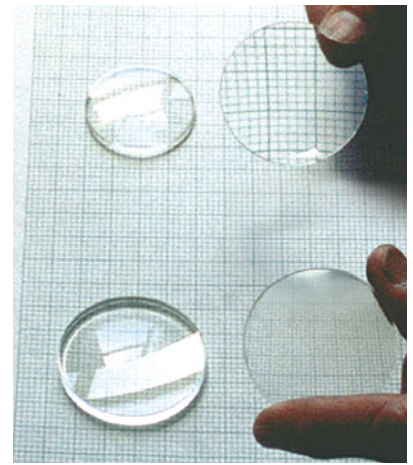
FIGURE 23–31 (a) Converging lenses and (b) diverging lenses, shown in cross section. Converging lenses are thicker at the center whereas diverging lenses are thicker at the edges. (c) Photo of a converging lens (on the left) and a diverging lens (right). (d) Converging lenses (above), and diverging lenses (below), lying flat, and raised off the paper to form images.
