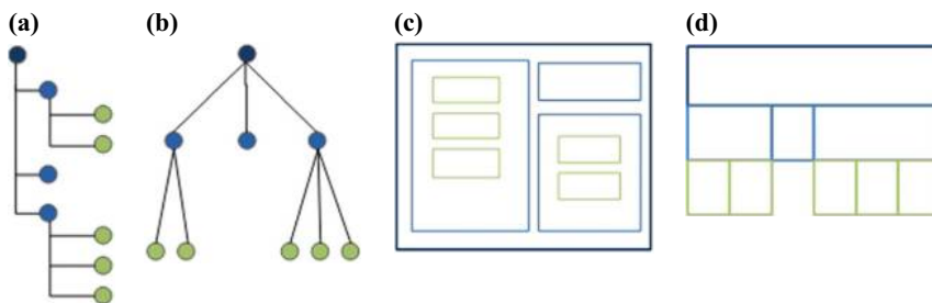
Notes: (a) Indented outline; (b) node-link graph; (c) nested containment; (d) alignment and adjacency. (a) and (b) belong to a node-link tree representation, while (c) and (d) present space-filling tree representations
