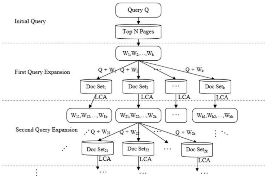
Figure 2. Methodology for extracting data from a limited accessible data source
