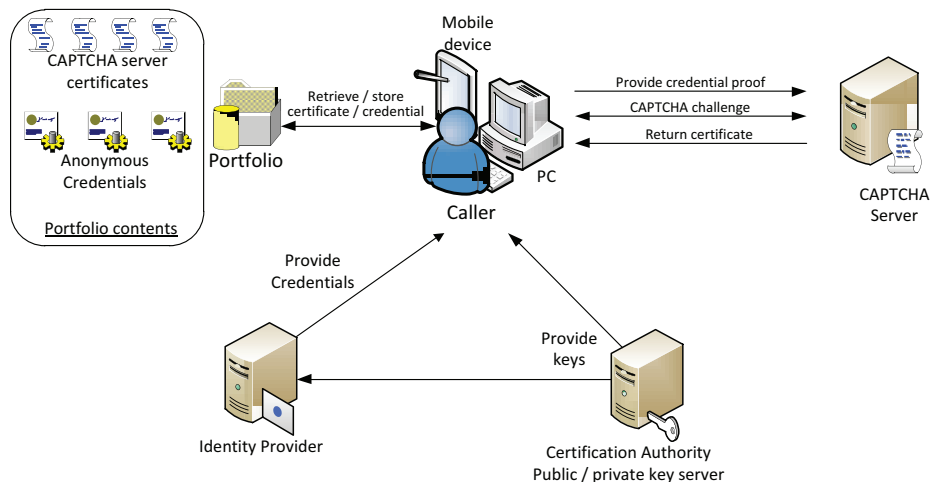
Figure 1. PrivCAPTCHA architecture
