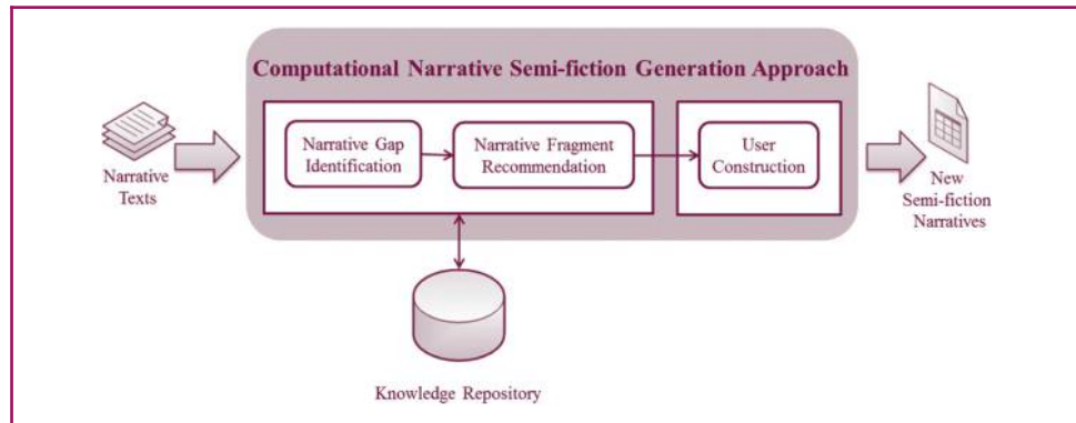
Figure 3 Framework of CNSG approach
