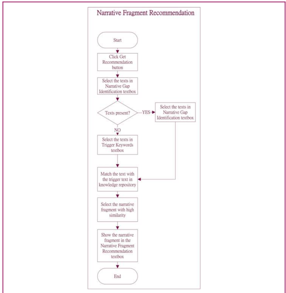
Figure 8 A workflow diagram of NFR
