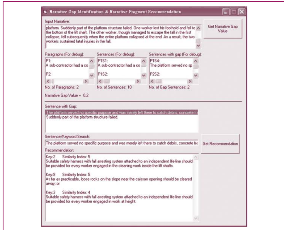
Figure 9 A snapshot of CNSG system for NFR
