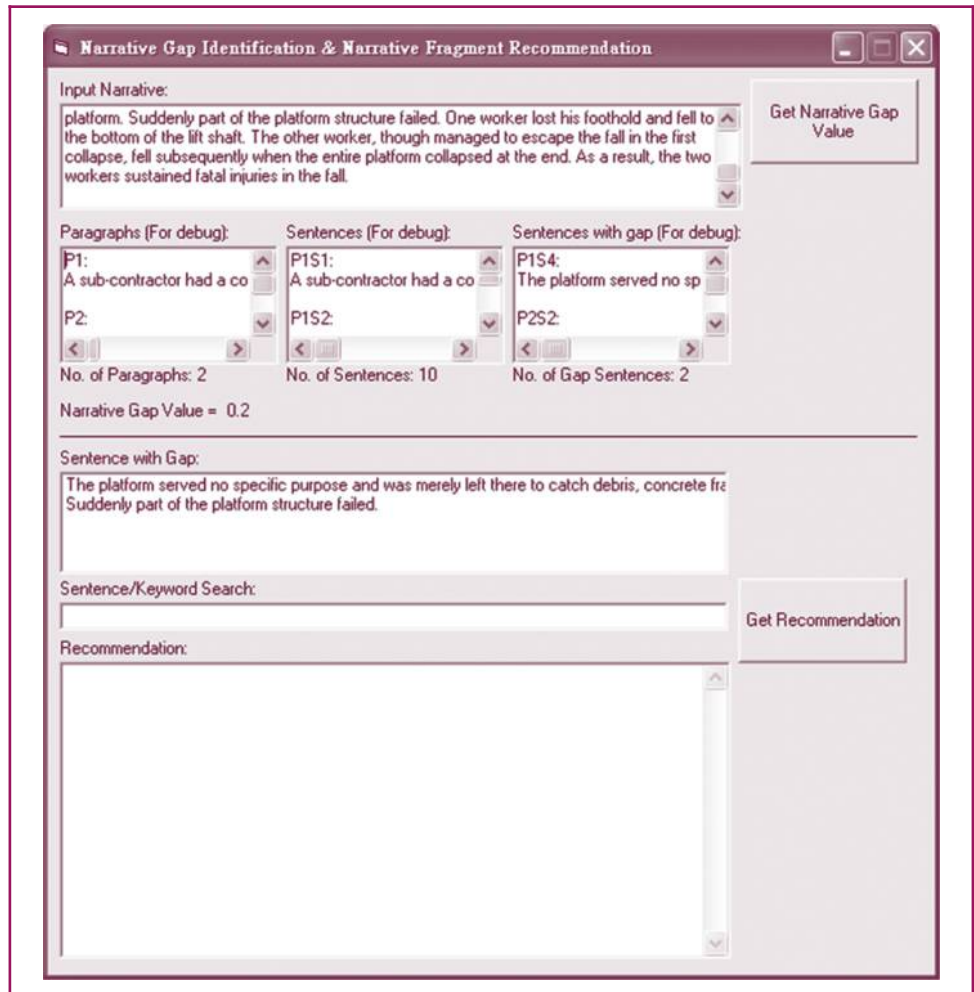
Figure 6 A snapshot of computational narrative generation system for NGI
