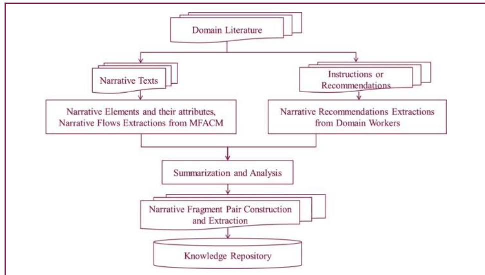
Figure 7 A schematic diagram of narrative fragment construction
