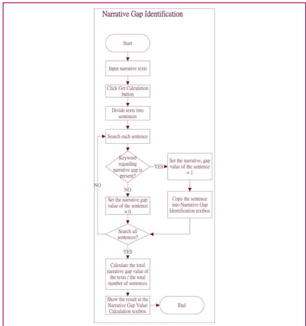
Figure 4 A workflow diagram of NGI
