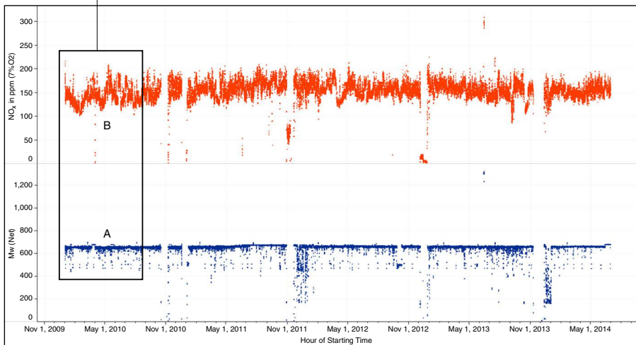
Figure 4. Energy output (MW) and the level of \text{NO}_x
