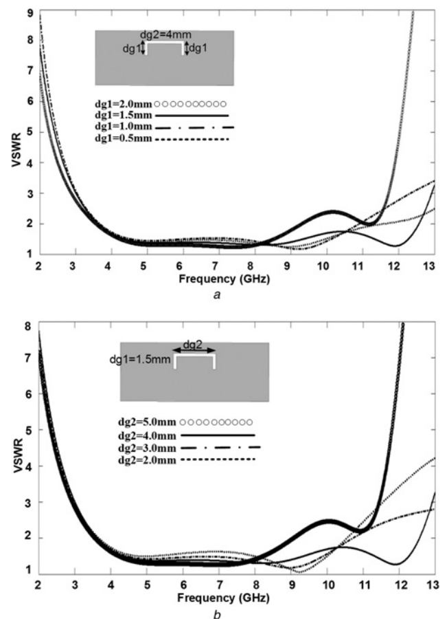
Fig. 3 Simulated VSWR characteristics of the antenna with an inverted U-shaped slot on the ground for different values of a dg1 b dg2
