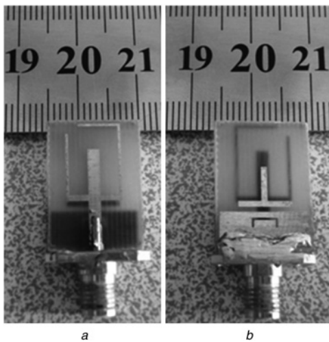
Fig. 9 Photo of the fabricated antenna
