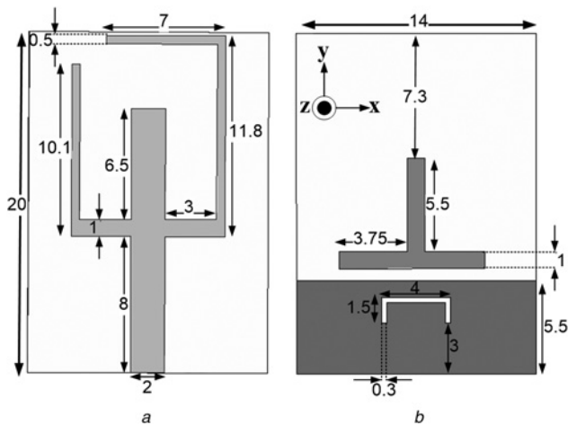
Fig. 1 Geometry of the suggested antenna and its values
