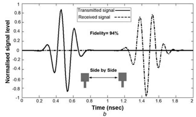
Fig. 12 Transmitted and received pulses for a UWB link with antennas without notches in
