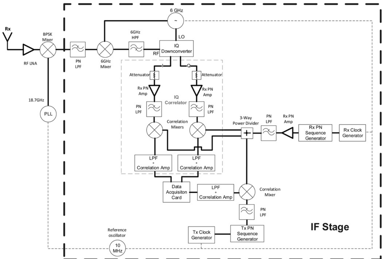
Fig. 3 Sounder receiver block
