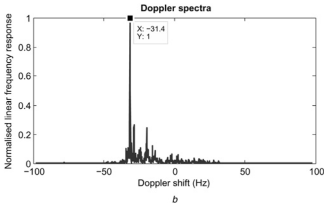
Fig. 7 Doppler spectra measurements
