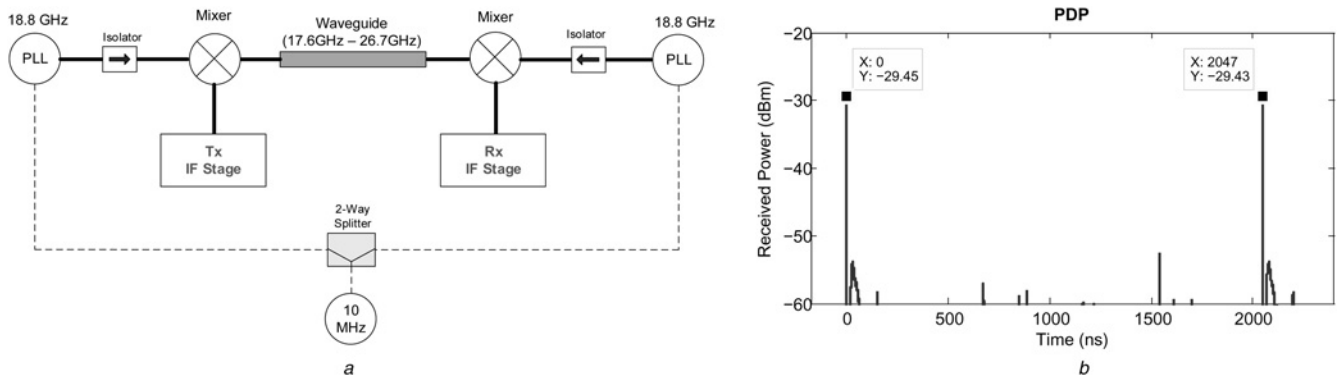
Fig. 6 Testing of fully integrated sounder
