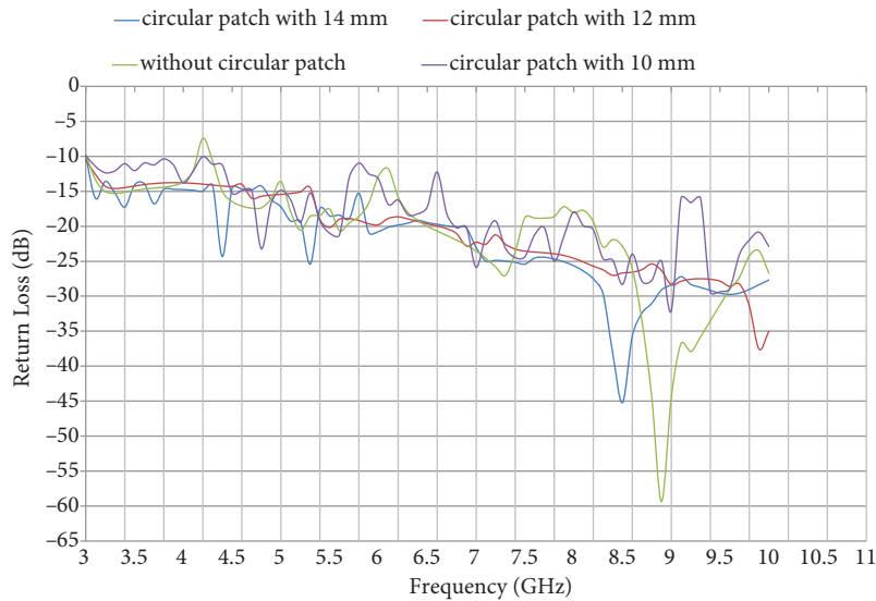
Figure 7. Simulated reflection coefficient versus frequency with different values of circular patch.
