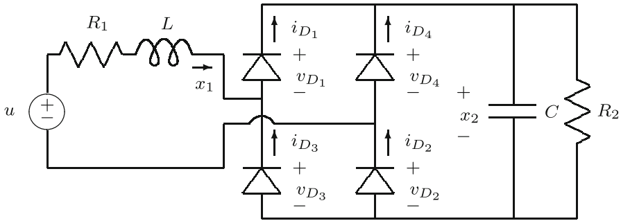
Fig. 1 Power converter diode bridge
