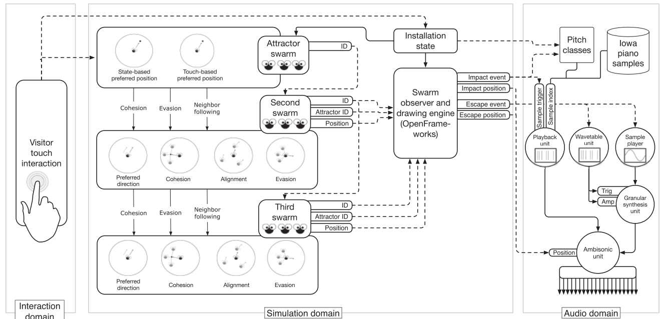
Figure 1. Schema for the swarm simulation of the piece Impacts . Here the three swarms are in a hierarchical relationship. Their continuous state change is analyzed in order
