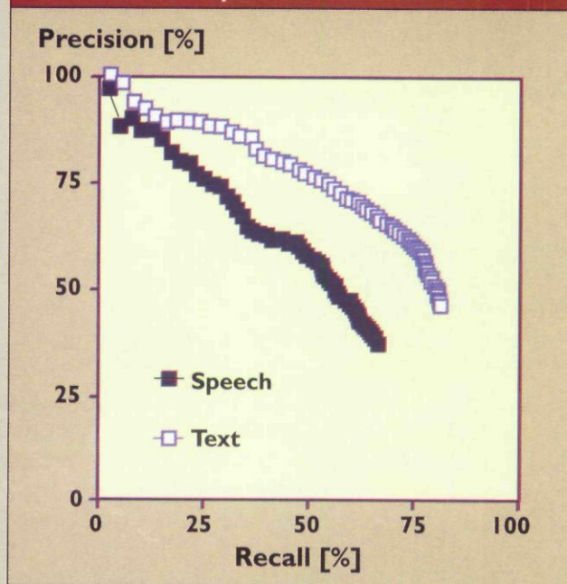
Figure 3. Topic-word extraction from broadcast news speech or news text.
