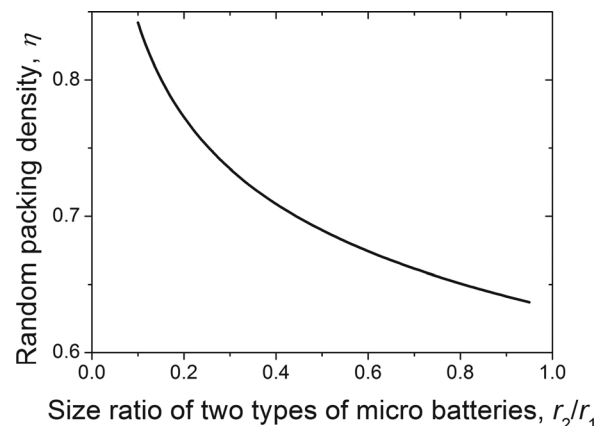
FIG. 3. Random packing density of a system with two types of micro batteries of different sizes. Their size ratio affects the random packing density.
