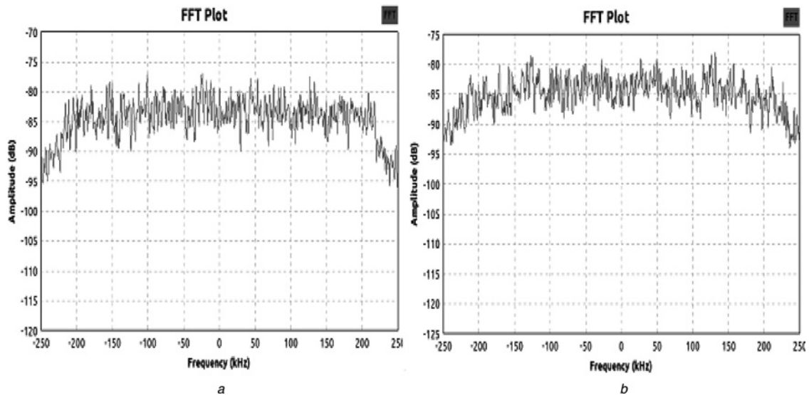
Fig. 13 FFT plots obtained by USRP N210 Rx for a Without PAPR reduction technique b With Phase modulation PAPR reduction technique
