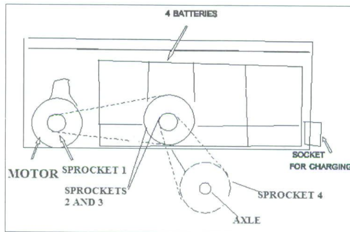
FIGURE 2B: Side View Showing Transmission
