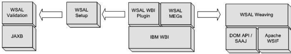
Fig. 6. WSAL weaver architecture.
