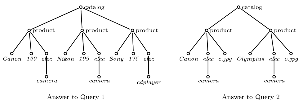
Fig. 6. Possible answers to queries 1 and 2. In order to improve readability, we omitted labels of leaves (obvious from the context) and depicted in italics the data value associated with each node.
