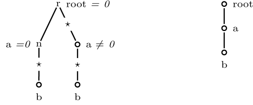
Fig. 7. The incomplete tree \mathbf{T} (to the left) and the query q (to the right).
