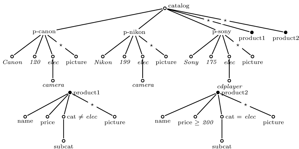
Fig. 8. The incomplete tree after Query 1. We omitted some labels when a data value is present and the label is clear from the context.
