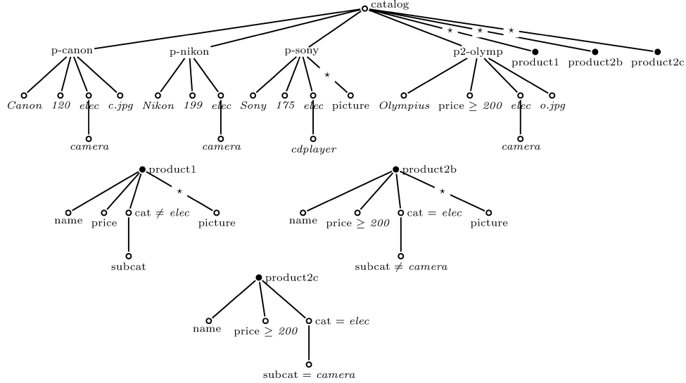
Fig. 9. The incomplete tree after Query 2.
