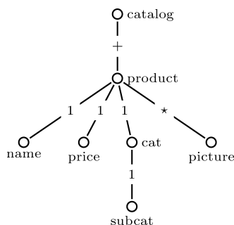
Fig. 1. The tree type for the catalog example.
