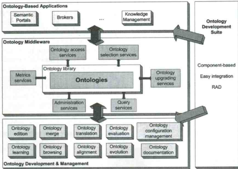
Fig. 3 Architecture of WebODE 2)
