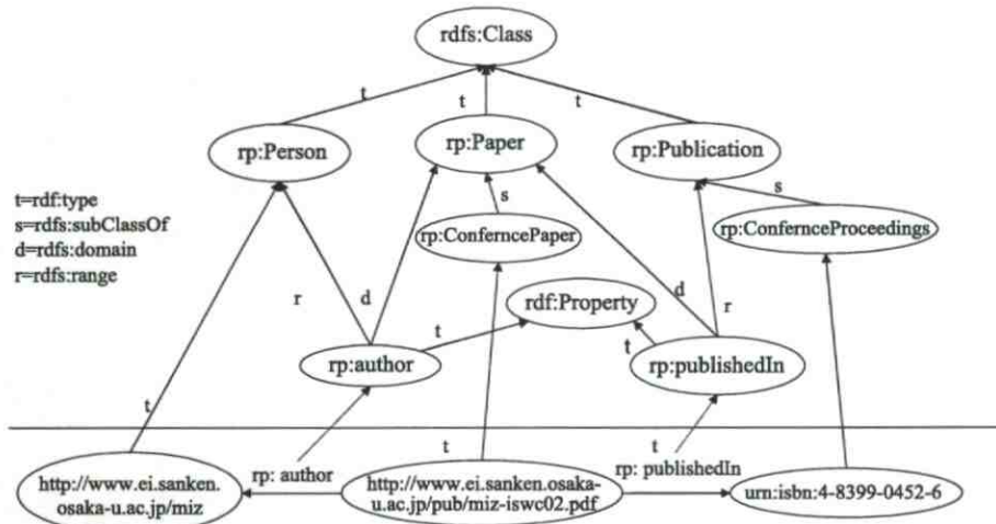
Fig. 2 A Simple Class Hierarchy of RDF Schema
