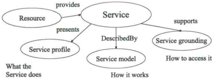
Fig. 9 Top-level Ontology of DAML-S 4)
