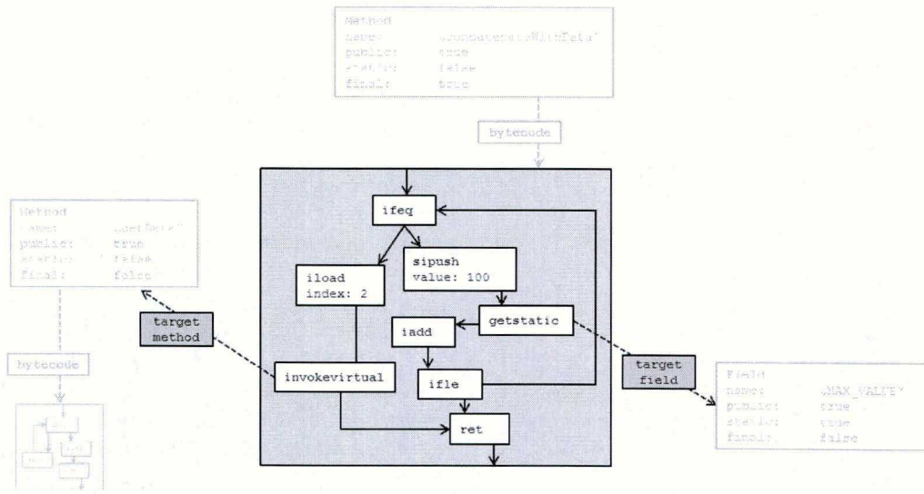
Fig. 5. Sample instruction execution graph shown in the context of objects it uses
