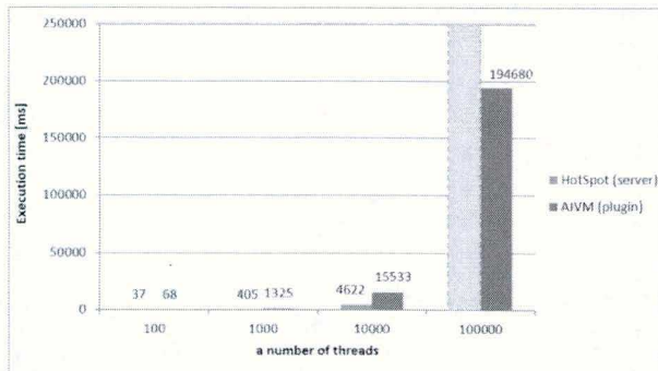
Fig. 15. Execution time of the test 5 – executing significant amount of concurrent threads
