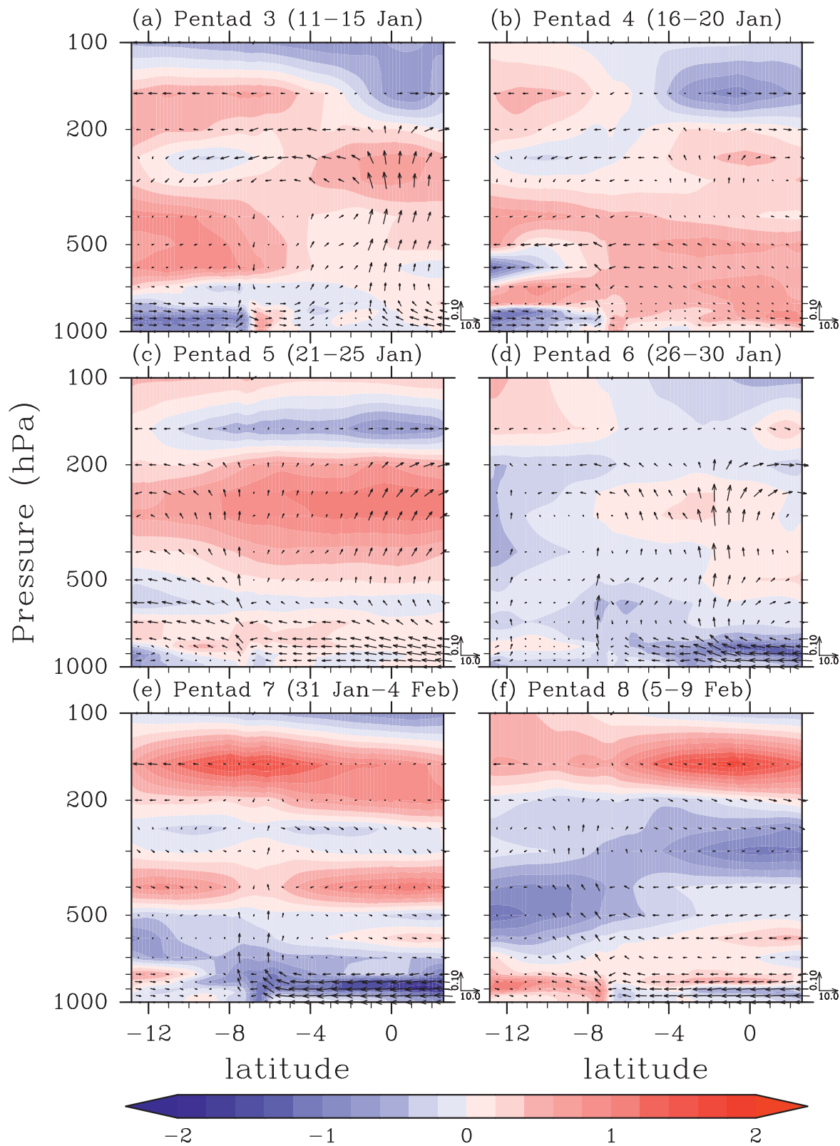
FIG. 8. Latitude–height cross sections of the ensemble mean of the model-simulated temperature anomaly from the two-month average (color; °C), and meridional and vertical winds (arrows; \text{m s}^{-1} ) averaged between 105.5^\circ and 108.5^\circ\text{E} for each pentad. Unit vectors ( 10 \text{ m s}^{-1} , 0.1 \text{ m s}^{-1} ) are shown on the bottom-right corner in each plot.
