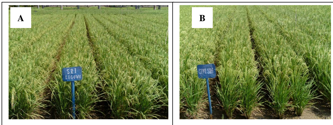
Figure 1. Performance of plant response against field spray application of bacterial consortium on rice cv. Sintanur under SRI practices. A= SRI treated using formulated bacterial consortium; B= semi –SRI practice treated using local microorganisms.
